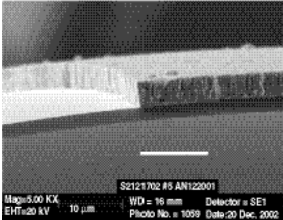
Fig. 3. SEM image of \sim 3 \mu\text{m} coating of W on a glass shell. This shell was coated using tapping agitation. The coating rate was \sim 0.7 \mu\text{m/hr} . The familiar columnar structure seen in sputter coatings is visible.
