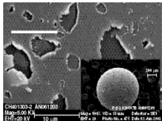
Fig. 2. SEM image of \sim 0.5\ \mu\text{m} palladium coating on glass shells. The shells were forced to move during the run by tapping on the bounce pan. Tearing of the palladium coating from the shells is seen, although it is less than what was observed with gold shells. The inset shows the full shell. Bar is 10\ \mu\text{m} .
