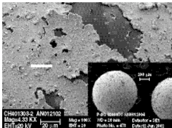
Fig. 1. SEM image of \sim 0.5\ \mu\text{m} gold coating on glass shells. The shells were forced to move during the run by tapping on the bounce pan. Major tearing of the gold coating from the shells is seen. The inset shows the full shell. Bar is 20\ \mu\text{m} .
