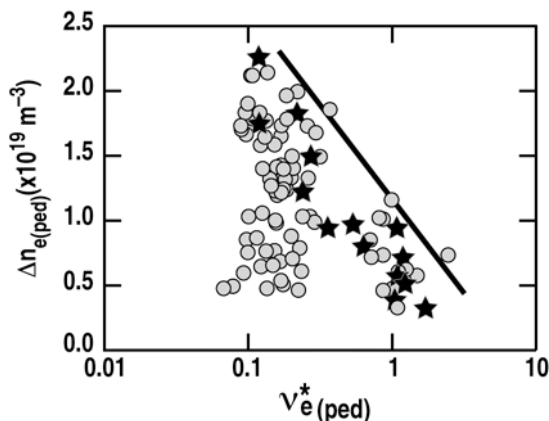
Fig. 3. Comparison of the pump-out magnitude, \Delta n_e , to the collisionality at the pedestal, \nu_{e(\text{ped})}^* . The line is only to guide the reader's eye and each point is for an individual RMP discharge. Symbols marked ( \star ) are given to indicate discharges used in later analysis, see figure 5.
