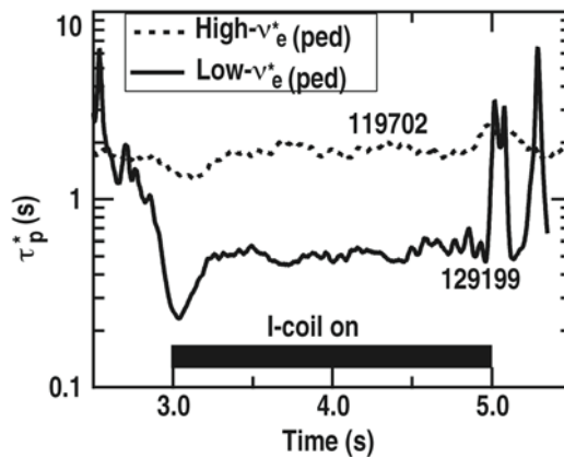
Fig. 4. Time history comparison of \tau_p^* from (2) discharges. One has high- v_{e(ped)}^* (119702) and the other has low- v_{e(ped)}^* (129199). The time-base has been normalized to the I_{coil} turn-on for 129199.
