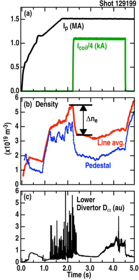
Fig. 1. (a) Plasma current, I_p , and RMP perturbation strength as denoted by the I_{coil} current, (b) density as measured by a CO_2 laser interferometer (labeled line avg.) and edge TS array (labeled pedestal) showing a large density drop ( \Delta n_e ) when the I_{coil} turns on, (c) lower divertor D_\alpha signal from the OSP.
