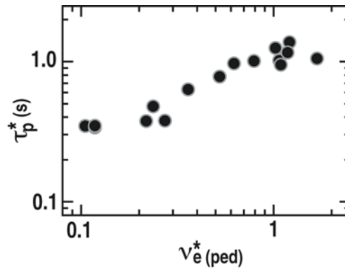
Fig. 5. Comparison of \tau_p^* versus v_{e(\text{ped})}^* during the pump-out phase of a number of RMP discharges.
