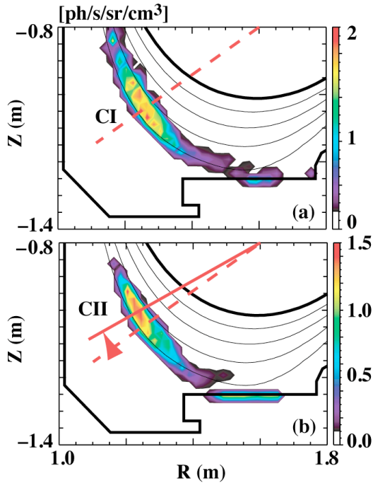
Fig. 2. 2-D intensity distributions of (a) CI (910 nm) and (b) CII (515 nm) emission in the crown during CD_4 injection. The red lines indicate the poloidal shift of the peak CII emission against the CI emission.
