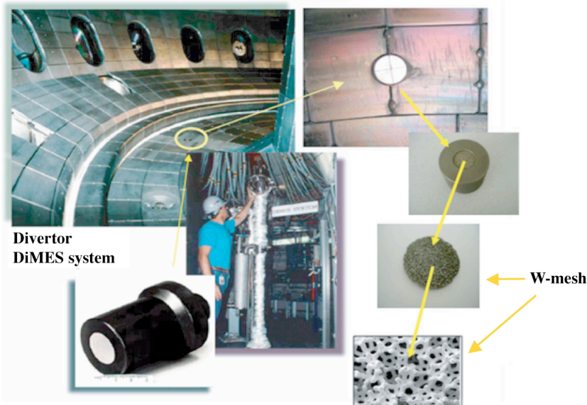
Fig. 1. BW-mesh concept can be tested with the DiMES system in DIII-D.
