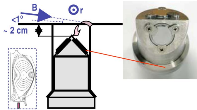
Fig. 2. Illustration and picture of DiMES mirror sample.
