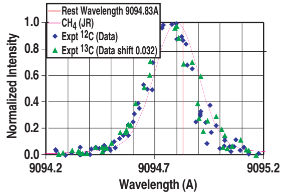
Fig. 3. Comparison of CI-9094.83A experimental and modeled line profiles. MDS Track 11 data for all H-mode data from the 2005 ^{13}\text{CH}_4 experiment and the previous set-up day that used ^{12}\text{CH}_4 . The ^{13}\text{C} experimental results have been shifted by 0.032 \text{ \AA} to account for differences between the base wavelength for this transition in ^{12}\text{C} and ^{13}\text{C} .
