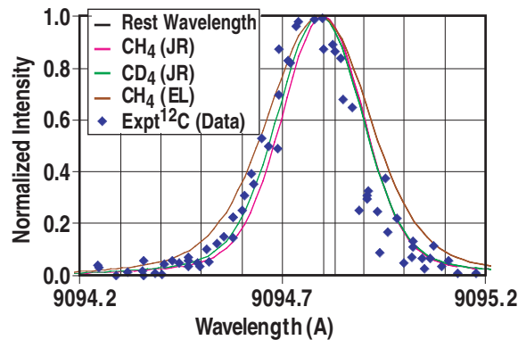
Fig. 5. Changes in the calculate line profiles resulting from different databases for the methane breakup processes and different hydrogen isotope masses. The ^{12}\text{CH}_4 experimental data from Fig. 3 are included for reference. The code-calculated profiles are convolved with the MDS instrument function.
