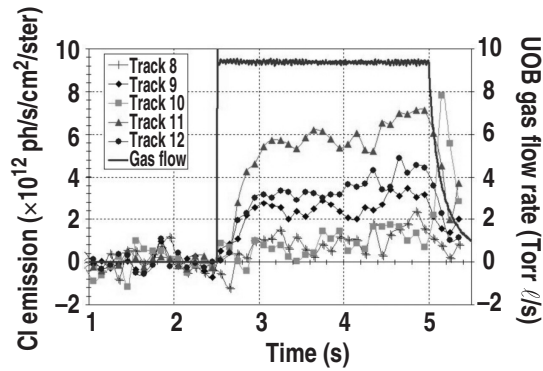
Fig. 2. Gas flow and integrated Cl emission is shown vs time for a sample L-mode, reversed-B shot with puffing from the toroidal pumping plenum (UOB). The zero for the emission scale is set by the average pre-puff (2–2.5 s) values. Emission intensity comes to steady state after ~0.5 s of gas flow due to the length of line between the gas supply and the vessel. Track 11, viewing the plenum exit, is found to have the greatest Cl intensity and track 10, viewing across midplane, the least.
