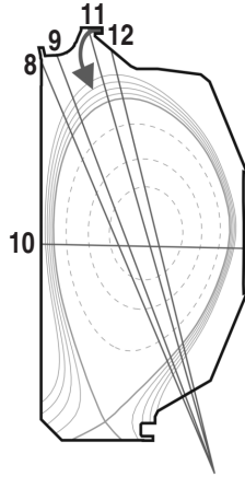
Fig. 1. Five viewing-lines of the spectrometer (MDS). Methane was injected toroidally symmetrically at the top of the vessel.
