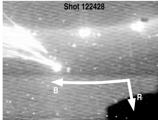
Fig. 5. Dust tracks recorded by DiMES TV with near IR filter. Dust holder is the bright spot where the tracks originate.
