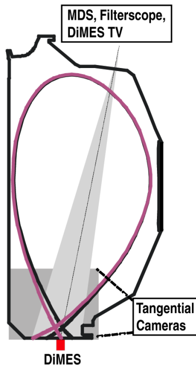
Fig. 2. Dust exposure geometry and diagnostic arrangement.
