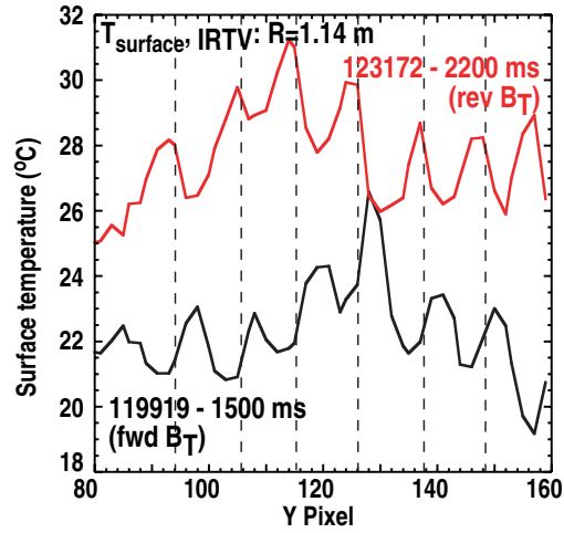
Fig. 3. Toroidal profiles of infra-red (IR) emission along the inner divertor (45 deg tiles) measured in forward (a) and reversed (b) B_T configuration. The radial profiles were taken at radial location R = 1.14 m. The vertical lines indicate tile gaps along the inner divertor.
