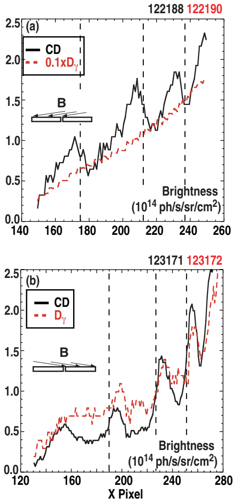
Fig. 2. Toroidal CD and D_\gamma emission profile along the inner divertor (45 deg tiles) obtained in forward (a) and reversed (b) B_T configuration. In forward B_T the profile was taken at radial location R = 1.03 m, in reversed B_T at R = 1.14 m, leading to slightly different locations of the tile gaps (vertical lines) on the (X,Y) image grid. The inserts show the alignment of the (total) magnetic field vector, \mathbf{B} , with respect to the tile surface.
