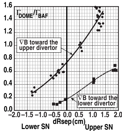
Fig.2. The ratio \Gamma_{\text{DOME}}/\Gamma_{\text{BAF}} depends on dR_{\text{sep}} for cases where the B \times \nabla B direction is toward the upper divertor (solid circles) and toward the lower divertor (solid squares).
