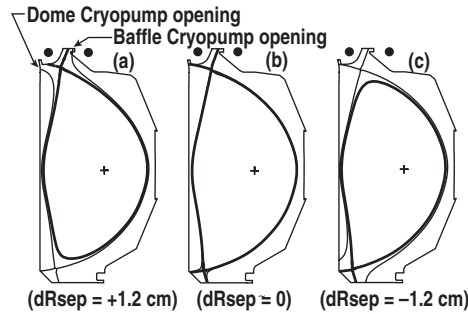
Fig. 1. The three basic equilibria used in this study: (a) DN biased toward the upper divertor ( dR_{\text{sep}} = +1.2 \text{ cm} ), (b) balanced DN ( dR_{\text{sep}} = 0 ), and (c) DN biased toward the lower divertor ( dR_{\text{sep}} = -1.2 \text{ cm} ). The “dome” and “baffle” pumps exhaust particles at the upper inner leg divertor target and upper outer leg divertor target, respectively. The “primary” separatrix is shown as a heavy line; the secondary separatrix is shown as a lighter line. Characteristic parameters: I_p = 1.2 \text{ MA} , |B_T| = 1.85 \text{ T} , and P_{\text{INJ}} = 6-11 \text{ MW} .
