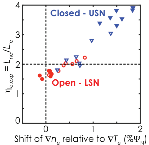
Figure 12. Variation of \eta_e at maximum pedestal electron pressure gradient in open (red) and closed (blue) divertor geometries vs the difference between locations of maxima of n_e and T_e gradients. Filled symbols are for partially detached divertors.
