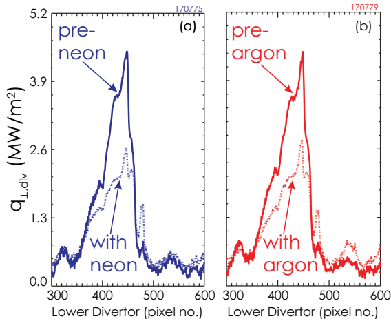
Figure 26. Lower divertor heat flux, measuring by an IR camera, for high- \beta_N hybrid scenario with and without (a) neon injection (3.60 Torr l/s) and (b) argon injection (1.54 Torr l/s).
