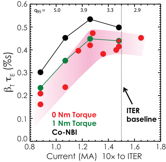
Figure 22. Fusion gain metric ( \beta\tau_E ) as a function of plasma current (lower abscissa) and safety factor (upper abscissa) for different levels of injected beam torque.
