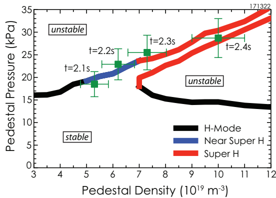
Figure 20. EPED prediction of pedestal pressure as a function of density based on high triangularity ( \delta=0.62 ), I_p=1.6 MA discharge. Green symbols are measured values.
