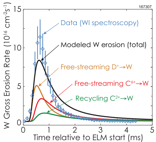
Figure 10. FSRM predictions of the gross erosion rate of tungsten vs. ELM time with the contributions from different W erosion pathways identified. Measurements inferred from W-I spectroscopy are overlaid (blue diamonds).
