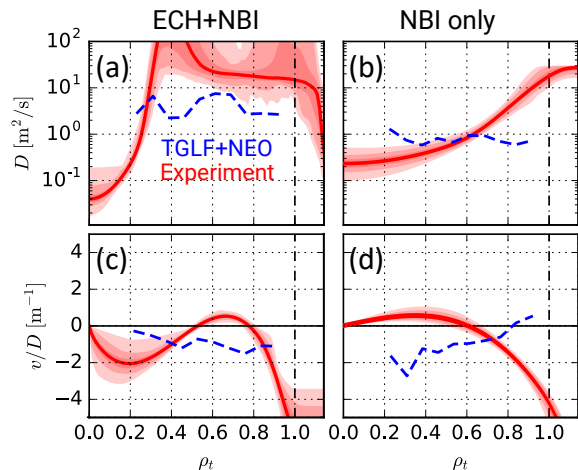
Figure 5. Measured [(a),(b)] aluminum diffusion and [(c),(d)] density peaking factor (red lines) for ECH+NBI with T_e/T_i=1.6 and NBI only with T_e/T_i=0.7 . Modeled aluminum transport from TGLF and NEO are also indicated (dash blue lines).
