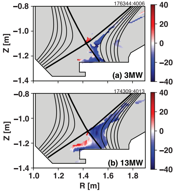
Figure 8. Coherence imaging spectroscopy of toroidal flow of C-III impurity for (a) 3 MW case and (b) 13 MW case. Negative flow velocity (blue) is towards the divertor target.
