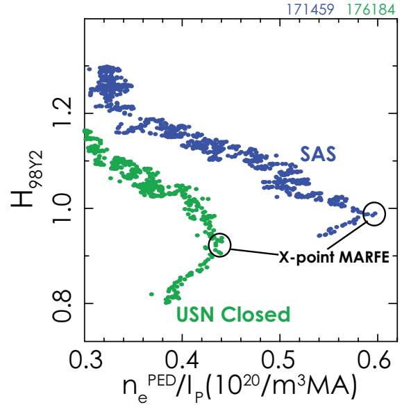
Figure 15. Comparison of IPB98(y,2) confinement factor vs. pedestal density normalized to plasma current for SAS (blue) and closed upper divertor (green). Densities for X-point MARFE formation are also indicated.
