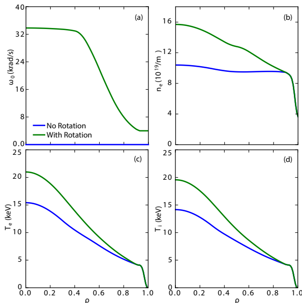
Figure 4. Predictions of ITER baseline scenario from TGYRO and TGLF, with and without \mathbf{E} \times \mathbf{B} shear effects: (a) toroidal rotation with 4 krad/s boundary condition, (b) electron density, (c) electron temperature and (d) ion temperature.
