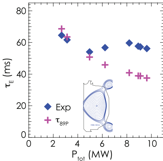
Figure 6. Measured energy confinement time (blue diamonds) vs. total heating power for negative triangularity discharges with an L-mode edge. The expected \tau_E from the ITER-89P confinement scaling relation (red crosses) is plotted for reference.
