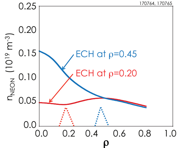
Figure 25. Comparison of neon impurity densities for high- \beta_N hybrid scenario with near-axis and off-axis ECH deposition and trace neon flow ( \sim 0.6 Torr l/s).
