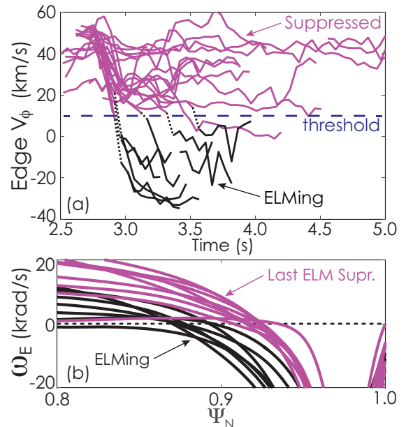
Figure 17. Low-torque ISS with applied n=3 RMP showing ELM and ELM-suppresses cases: (a) edge rotation of carbon impurity, and (b) \mathbf{E} \times \mathbf{B} rotation profile vs. normalized poloidal flux.
