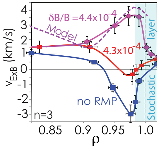
Figure 18. \mathbf{E} \times \mathbf{B} velocity profile before L-H transition, as measured by DBS, with and without applied RMP. The expected edge magnetic stochastic layer is shaded. Dash line shows predicted \mathbf{E} \times \mathbf{B} velocity from a simple fluid model of stochasticity for the largest \delta B/B case.
