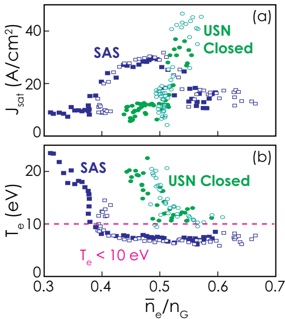
Figure 14. Comparison of (a) Langmuir probe ion saturation current density and (b) electron temperature near strike point vs. line-averaged density normalized to the Greenwald density limit for SAS (blue) and closed upper divertor (green).
