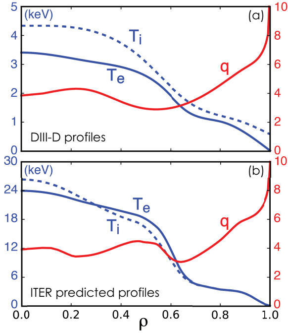
Figure 24. Electron temperature, ion temperature and safety factor for high \beta_P scenario with q_{95}\sim 6 : (a) measured profiles from DIII-D discharge with strong ITB, and (b) TGYRO prediction for ITER steady-state scenario with zero E \times B shear.
