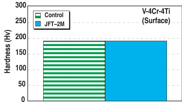
Fig. 5. Hardness of the V-4Cr-4Ti specimen surface before and after the tokamak exposure.
