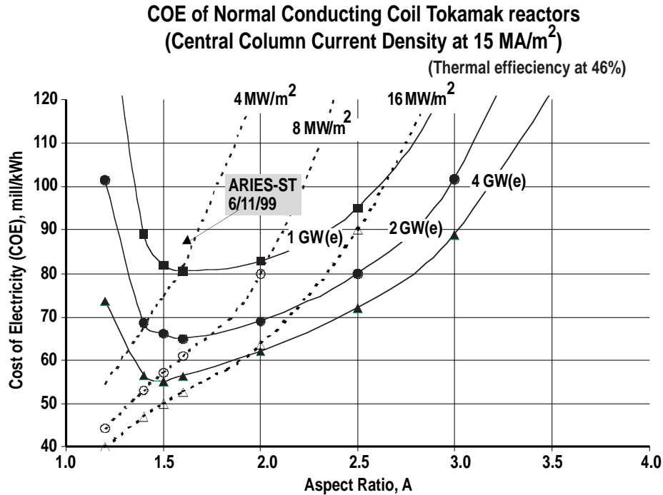
Fig. 1. COE of normal conducting coil tokamak reactor designs.
