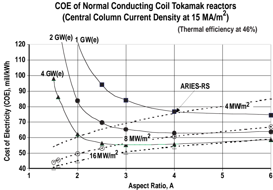
Fig. 2. COE of superconducting coil tokamak reactor designs.
