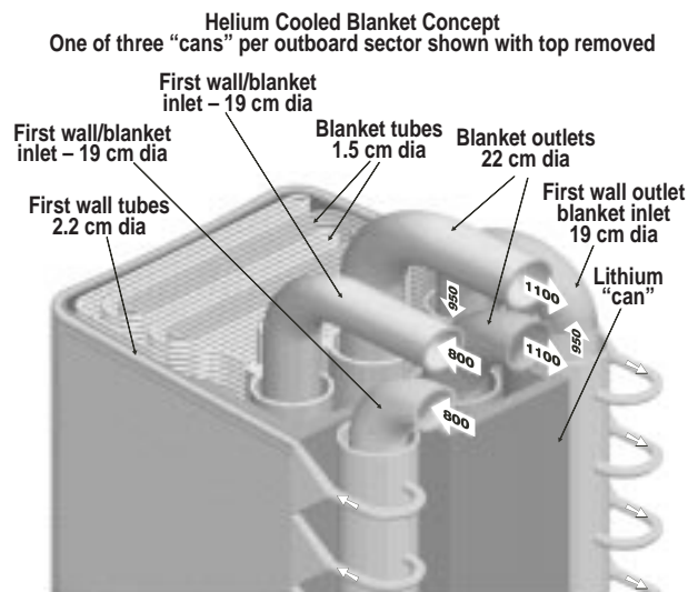
Fig. 4. W-alloy helium-cooled blanket concept.
