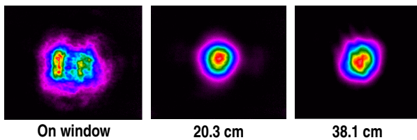
Figure 2. Infrared measurements of the beam from the diode gyrotron, Katya, as a function of distance from the BN output window.
