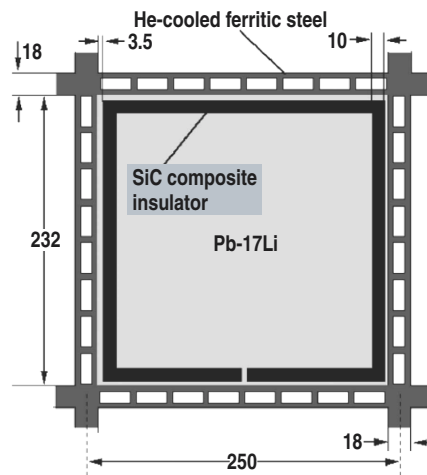
Fig. 1. Cross section of the Pb-17Li breeder unit cell of DCLL (dimensions are in mm).
