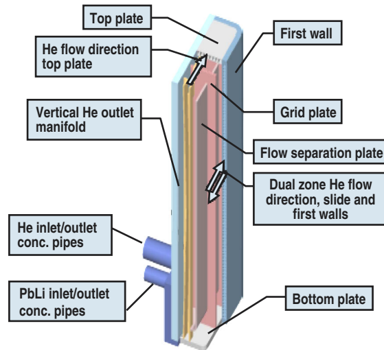
Fig. 3. DCLL ITER-TBM module design schematic.
