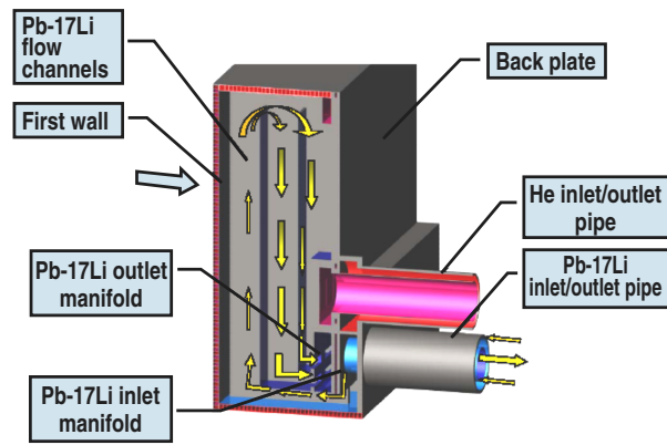
Fig. 2. DCLL configuration for the Reference Tokamak Reactor Design.
