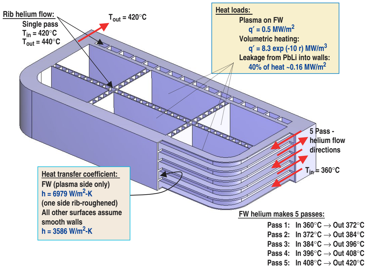
Fig. 4. Counterflow helium cooled TBM first wall and corresponding input and output parameters.
