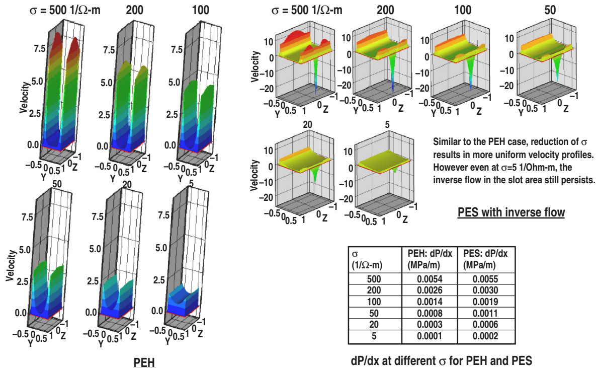
Fig. 5. Pb-17Li flow distribution in the flow channel as a function of electrical conductivity of SiC-composite FCI for the cases of PES and PEH. (Magnetic field is applied in the z-direction and velocity is in m/s.)
