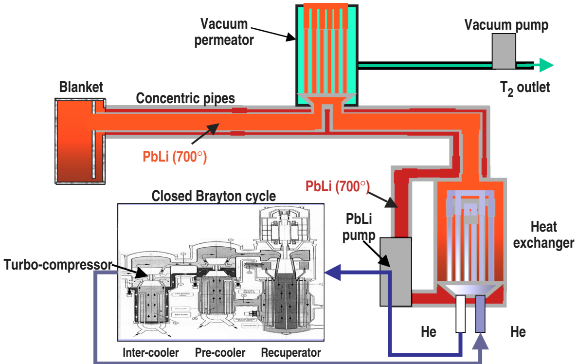
Fig. 6. The Pb-17Li loop showing the concentric tubes, the vacuum permeator for tritium extraction and the PbLi to helium heat exchange.
