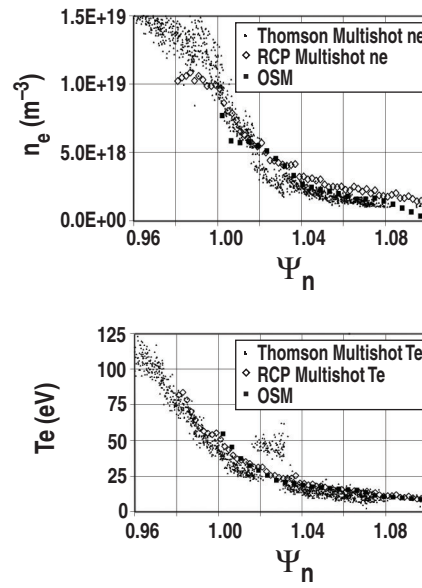
Fig. 3. Profiles of n_e and T_e in the SOL, from [7].
