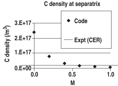
Fig. 6. Carbon density at the separatrix calculated by the code, compared with the CER measured value.
