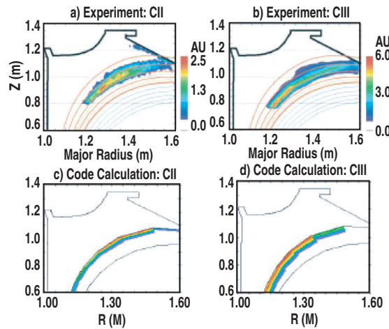
Fig. 2. Reconstructed 2D pictures from the toroidal viewing camera, in CII (top left) and CIII (top right). At bottom the same but for code results, case of M_{\parallel} = 0.4 and D_{\perp} = 0.3 \text{ m}^2/\text{s} . Same color bars for expt and code. Note that the camera CIII picture is occluded below Z \sim 0.8\text{m} .
