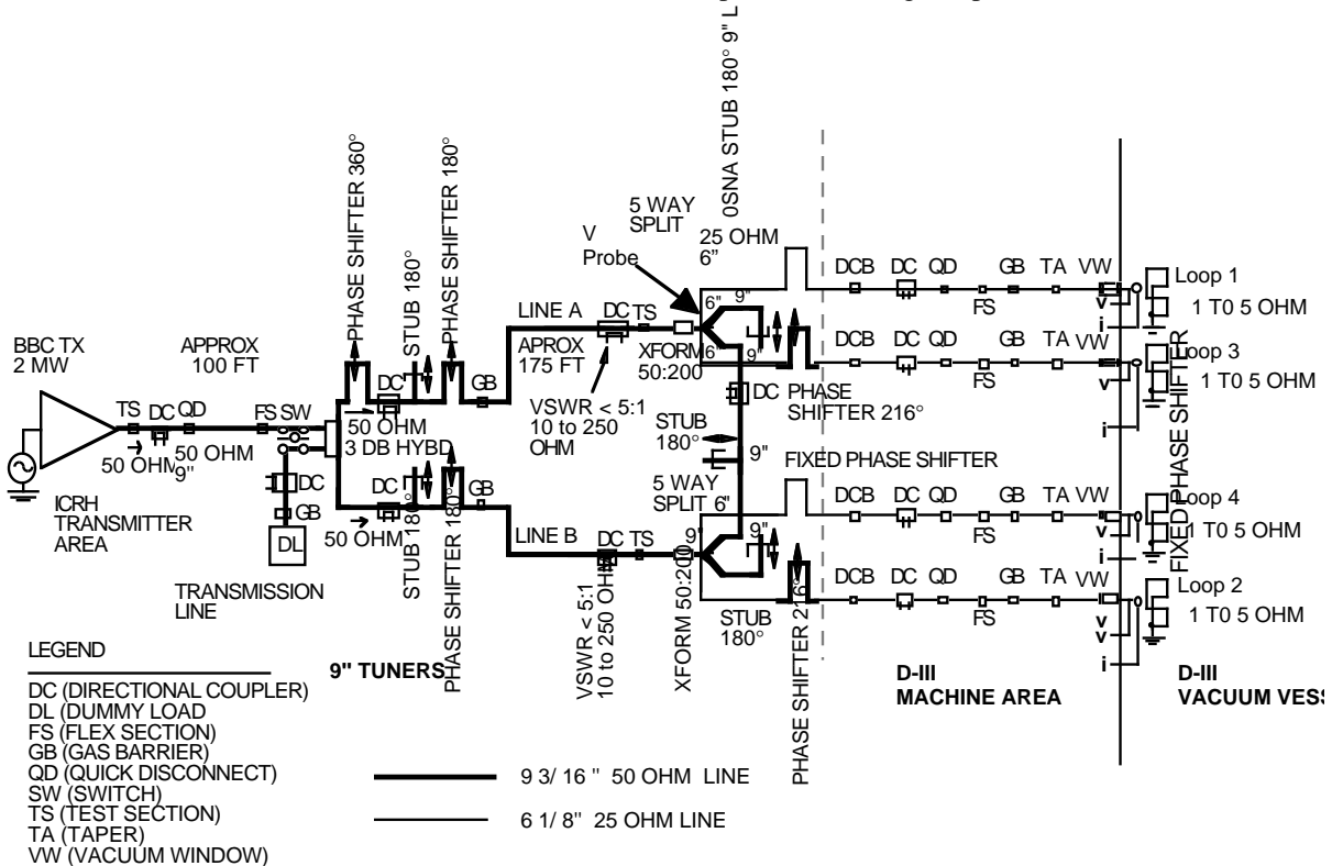
Fig. 1. DIII-D transmission line and antenna tuners
