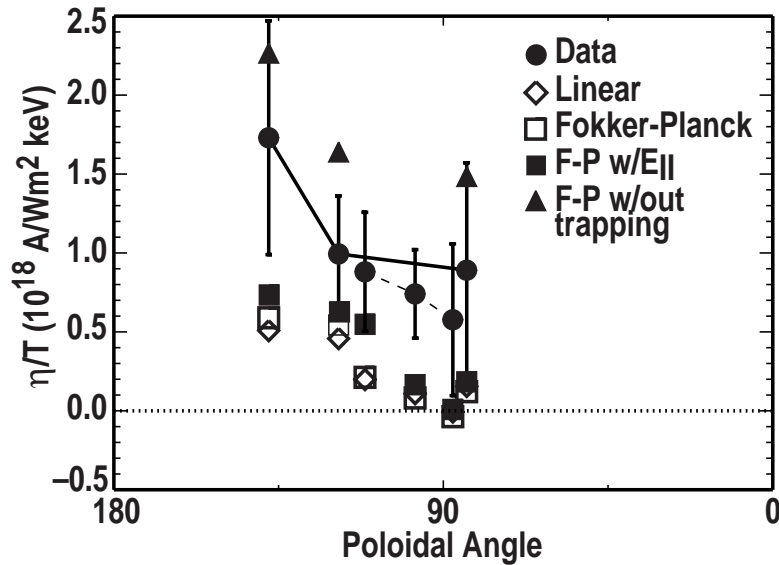
FIG. 5. Variation of normalized efficiency with poloidal angle at fixed \rho . The points connected by the solid line are \rho = 0.30-0.38 . The points connected by the dashed line are for \rho = 0.44-0.50 . Poloidal angle is defined as the angle with respect to the major radius with the magnetic axis as the origin. The outboard midplane is the 0^\circ reference, vertically above the axis is 90^\circ , and the inboard midplane is 180^\circ .
