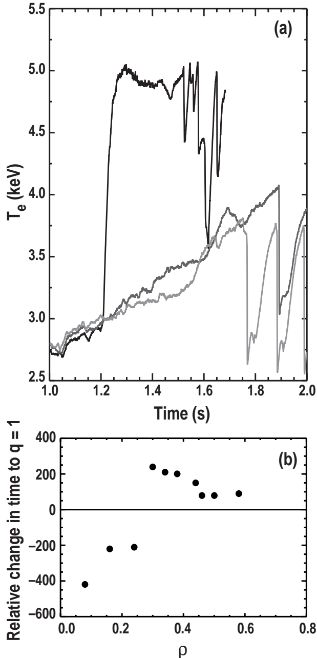
FIG. 2. (a) Time histories of central electron temperature. The first sharp drop in temperature in each trace signifies the time of the first sawtooth. The central ECCD case has the first sawtooth at 1.52 s while the off-axis case has the first sawtooth at 1.89 s. The NBI-only fiducial case has the first sawtooth at 1.74 s. Note that the sawteeth are also much more rapid in the central ECCD case. (b) A dataset of similar discharges (same q , density, and ECH power) showing the effect illustrated in (a) is systematic. Current drive inside of \rho = 0.3 hastens the onset of sawteeth while current drive for \rho > 0.3 delays the onset of sawteeth as discussed in the text.
