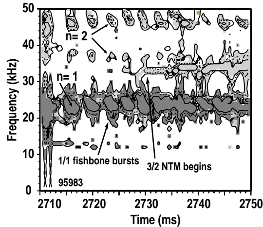
FIG. 10. Contours of constant B\text{-dot} mode amplitude for n=1 (dark shade) and n=2 (light shade) modes. A continuous 3/2 mode is triggered by a fishbone burst at 2730 ms.
