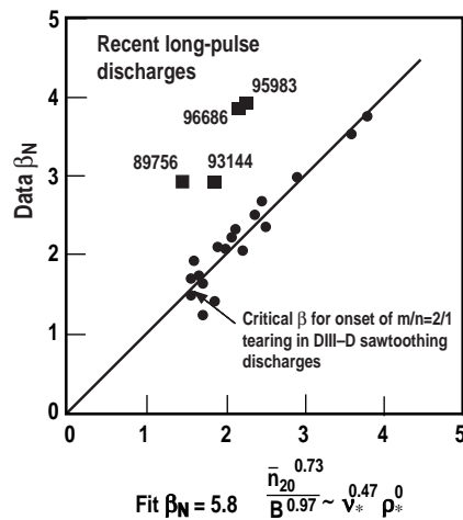
FIG. 11. The beta limit for discharges discussed in this paper (squares) exceed the NTM limit established for sawtoothing discharges (circles and line) by a factor of \sim 2 .
