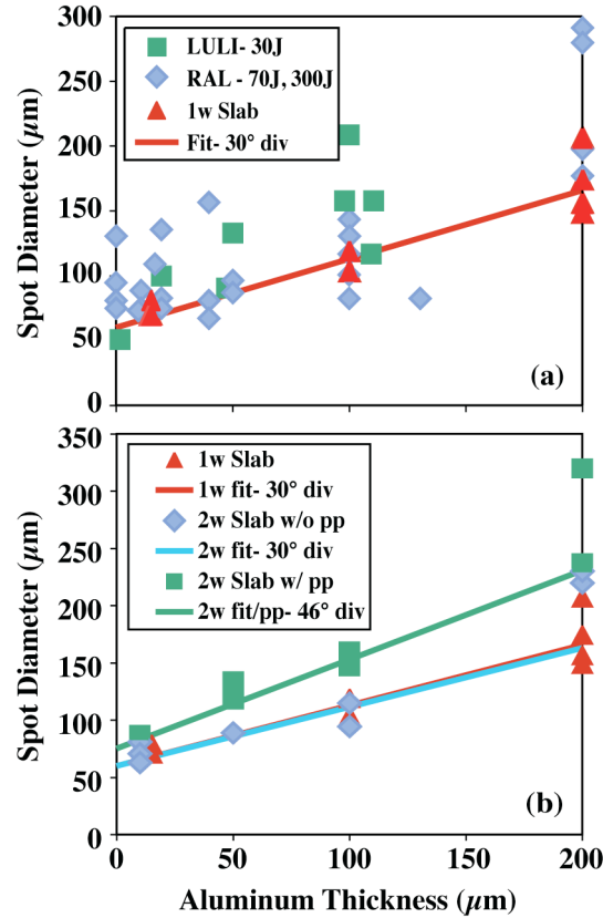
FIG. 1. fwhm of K_\alpha fluorescence from Cu layers buried in Al beneath the laser/plasma interface. (a) shows data at 1\omega and nominal prepulse overlain on historical divergence data [5]. (b) shows data at 2\omega with a prepulse added equivalent to that present in (a) and without prepulse. Lines and their slopes are guides to the eye, not fits.
