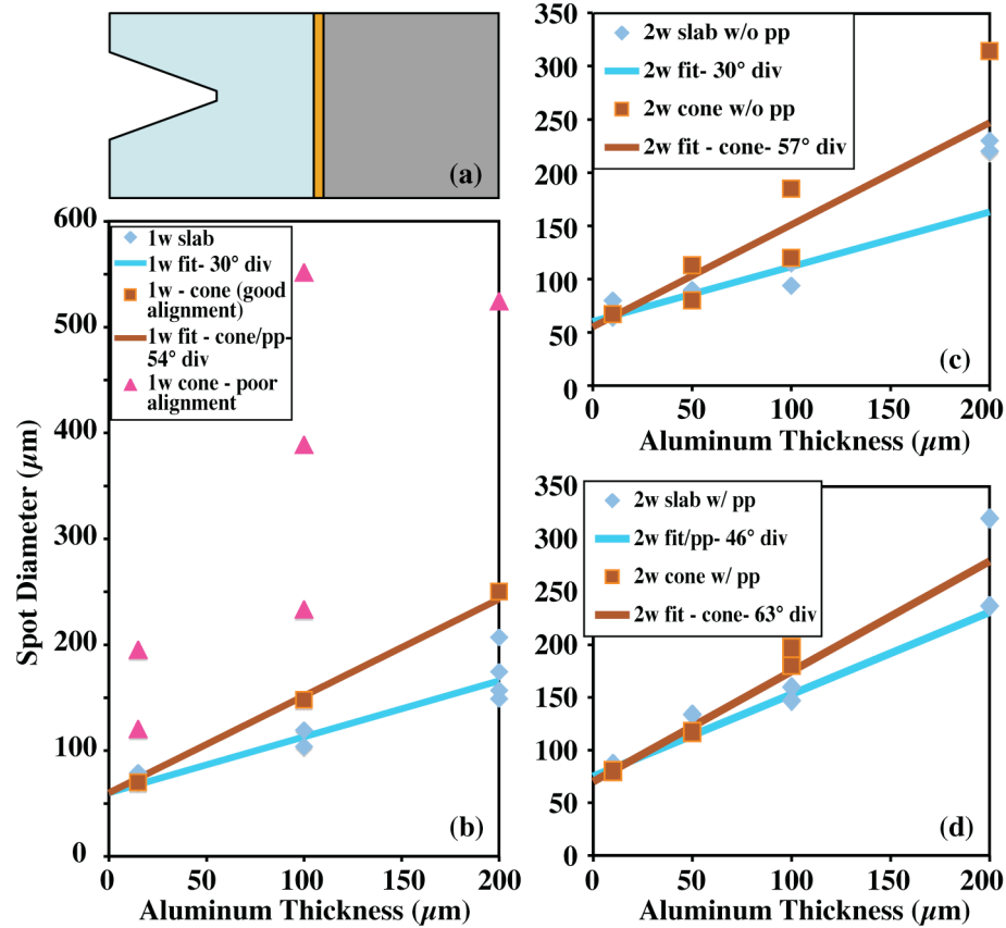
FIG. 2. (a) cross-section of 'buried cone' target. The cone has a 30 \mu\text{m} diameter flat at the bottom of a conical cavity in Al with 30° opening angle. The Cu layer is backed up by a 1 mm thick 'get-lost' layer of carbon or carbon-loaded plastic that ensures electrons make only one pass through the Cu. The graphs show fwhm fluorescent spot diameters for (b) 1 \omega laser pulses preceded by \sim 5 mJ prepulse, (c) 2 \omega laser pulses without prepulse, and (d) 2 \omega laser pulses with prepulse equivalent to that in (a). The blue diamonds are for flat laser/plasma interfaces, the brown squares for buried cone geometry, the red triangles for poorly aligned shots.
