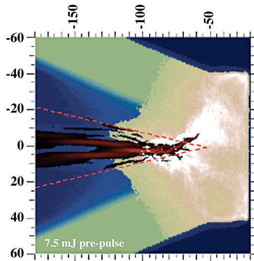
FIG. 3. Overlay of laser Poynting flux and electron density maps after 7.5 mJ of prepulse and 1 ps after nominal peak fluence on target (from Fig. 3 of MacPhee et al. [8]).
