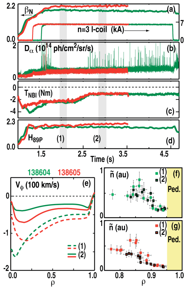
FIG. 4. Effects of NBI torque ramp down in discharges with different values of \beta_N . The discharge in red (138605) is terminated early by a fault of the plasma control system. Time histories of: (a) \beta_N , I-coil current; (b) D_\alpha light; (c) NBI torque; (d) confinement quality. Shaded vertical bands labeled (1) and (2) indicate time ranges relevant to the next panels. (e) Radial profiles of toroidal plasma rotation averaged over the time ranges of turbulence measurement analysis, (1) and (2). Radial profiles of relative density fluctuation level measured by Doppler backscattering at high and low rotation in (f) discharge with lower \beta , and (g) discharge with higher \beta .
