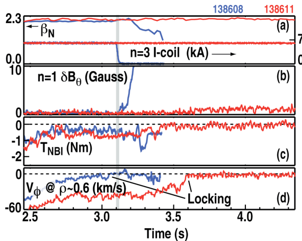
FIG. 6. Comparison of discharges with and without removal of the n = 3 NRMF during phase of low NBI torque. Time histories of: (a) \beta_N and I-coil current; (b) n=1 locked mode detector signal; (c) NBI torque; and (d) toroidal plasma rotation at the approximate location of the q = 2 surface.
