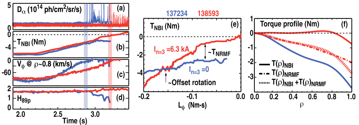
FIG. 2. Comparison of NBI torque rampdown discharges with constant NRMF applied (red traces, 6.3 kA of n = 3 I-coil current) and with no NRMF (blue traces). (a) Time histories of D_\alpha light, showing QH-mode regime when bursting behavior (from ELMs) is absent; (b) NBI torque; (c) plasma toroidal rotation at \rho \sim 0.8 ; (d) energy confinement quality. (e) Discharge trajectories in the plane of NBI torque versus total toroidal angular momentum. (f) Profiles of integrated torque density versus normalized minor radius calculated just before end of QH-mode phase [times indicated by vertical bands in (a)-(d)]. Only four curves are shown in (f) since T(\rho)_{\text{NRMF}} = 0 for the blue case.
