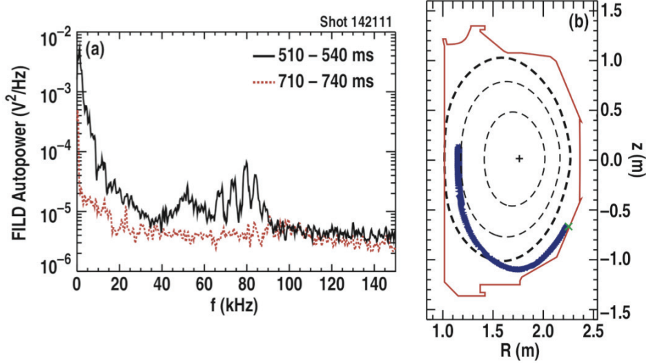
FIG. 6. Energetic ion loss measures from DIII-D discharge 142111. (a) Autopower spectrum from the FILD PMT signal averaged over 510 \leq t \leq 540 ms (solid black) and 710 \leq t \leq 740 ms (dotted red). (b) Trajectory of a typical loss orbit (solid blue trace) based on FILD camera data at t = 525 ms. The full orbit trajectory has been averaged to reduce the number of points plotted. Ion orbit properties are: E_o = 80 keV, v_{\parallel}/v = 0.676 ( 47.5^\circ ), FILD aperture position [R, z] = [2.252, -0.666] m (indicated by the green \times ).
