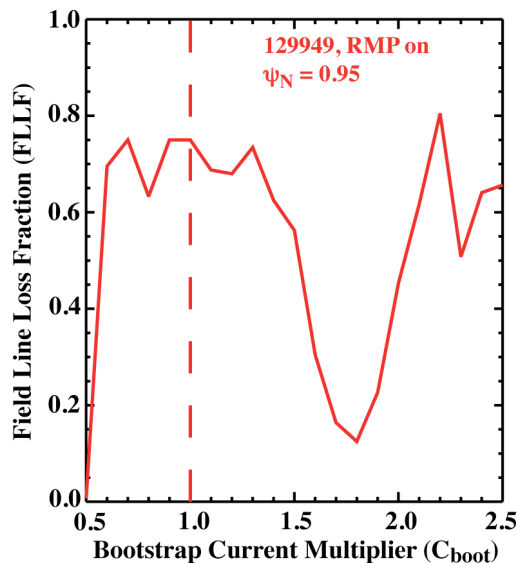
FIG. 10. Field line loss fraction vs. edge current multiplier. Experimental value is at C_{\text{boot}} = 1 (vertical dashed).
