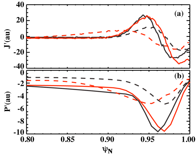
FIG. 6. (a) Current gradient and (b) pressure gradient for two discharges with different q_{95} values (3.6 in black, 4.1 in red/gray), before (solid) and after (dashed) RMP is applied [21].
