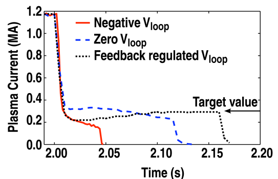
FIG. 7. RE current evolution for a different applied V_{loop} : negative (solid), zero (dashed) and feedback regulated (dotted) at I_{RE} = 300 kA.
