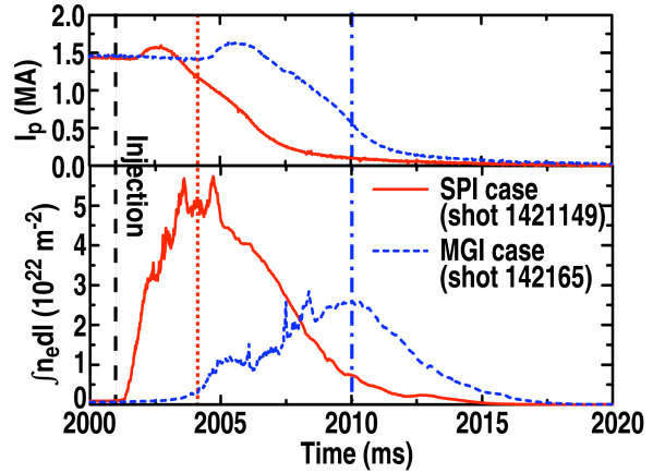
FIG. 4. Line-integrated density during SPI (solid) and MGI (dashed) rapid shutdown of an ohmic plasmas. The vertical lines show the time when the density starts to roll-over for the SPI (dot) and MGI (dash-dot).
