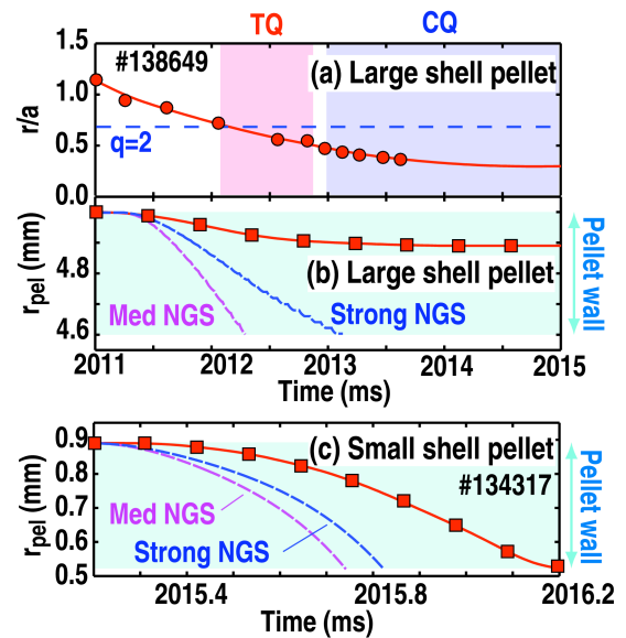
FIG. 5. (a) Pellet trajectories r/a as a function of time for a large shell pellet. Experimental (solid) and calculated (dash) pellet burnthrough of a large (b) and small (c) shell as a function of time.
