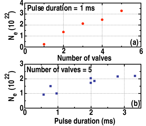
FIG. 1. MEDUSA-II gas quantity and plasma thermal energy variation experiments.
