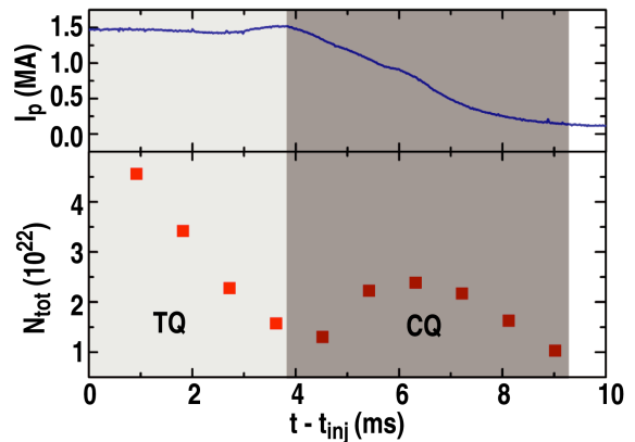
FIG. 3. Plasma current (upper) and N_{tot} (lower) during an SPI induced shutdown with thermal energy content of 1600 kJ ( t_{inj} being the injection time). The light shaded area shows the TQ phase and the dark shaded one the CQ phase.
