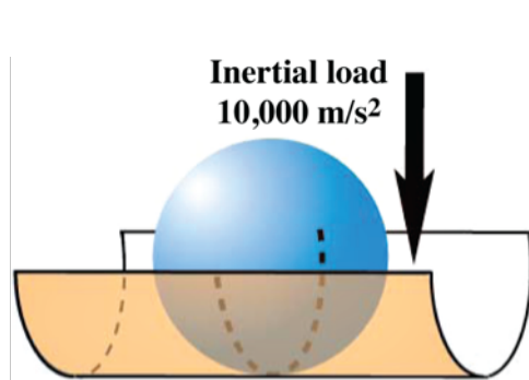
Fig. 6. A spherical pellet will form a line contact when bouncing down a tube or barrel.
