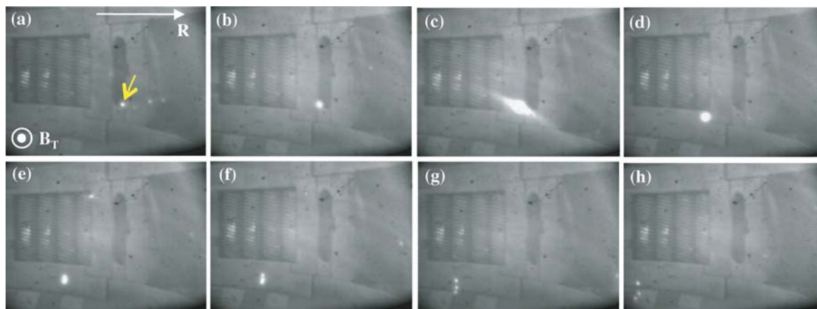
FIG. 2. Time history of a dust particle observed by the fast camera in the outboard DIII-D SOL.
