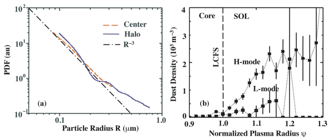
FIG. 1. Dust size distribution (a) and radial density profile (b) measured by Mie scattering.
