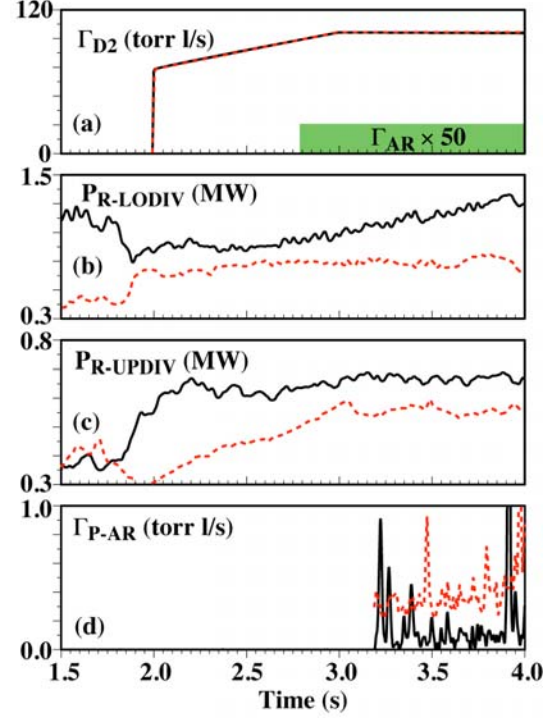
FIG. 5. Cases where the argon is injected into the lower divertor PFR of DN plasmas. Same waveforms as in Fig. 4
