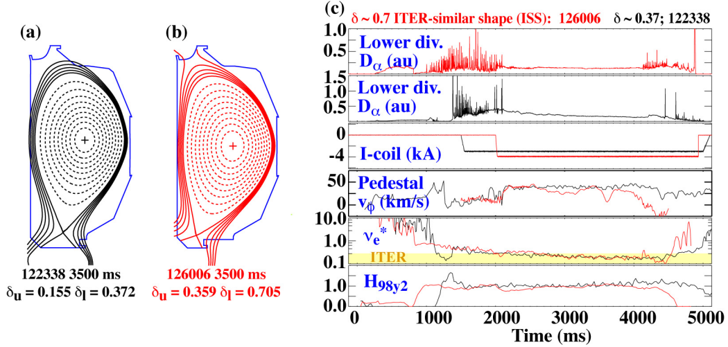
FIG. 3. Plasma shapes for the RMP ELM suppression experiments at v_e^* \sim 0.2 with (a) \delta \sim 0.37 and (b) \delta \sim 0.7 in an ITER-similar shape (ISS). (c) ELM suppression at v_e^* \sim 0.2 for the \delta \sim 0.37 (black) and \delta \sim 0.7 (red) shapes, showing, top to bottom: lower divertor recycling, I-coil current, pedestal toroidal rotation v_\phi , v_e^* , and H-mode confinement quality factor H_{98y2} .
