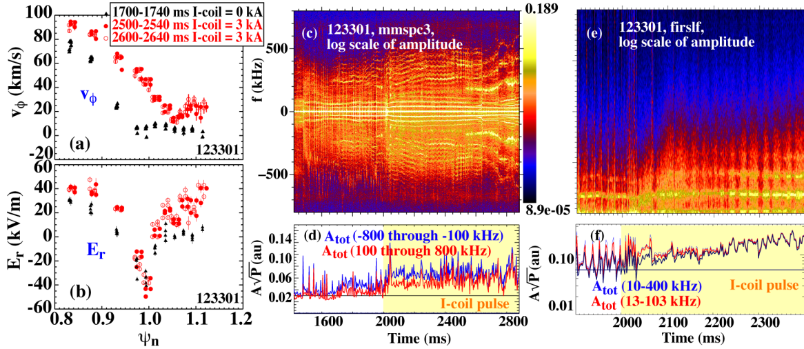
FIG. 7. Pedestal (a) v_\phi and (b) E_r profiles during the ELMing phase before the I-coil and at two times during the RMP-assisted ELM-free H-mode for discharge 123301 with \nu_e^* \sim 0.2 and \delta \sim 0.37 . (c) \tilde{n} amplitude spectrum and (d) rms amplitudes A_{\text{tot}} for frequencies (blue) < 0 kHz and (red) > 0 kHz versus time for k_\theta = 1 \pm 1 \text{ cm}^{-1} (FIR scattering). (e) \tilde{n} amplitude spectrum and (f) rms amplitudes for (blue) 10-400 kHz and (red) 13-103 kHz for a channel reflecting at n_e = 1.3 \times 10^{13} \text{ cm}^{-3} ( \psi_n = 0.98 ) in the pedestal.
