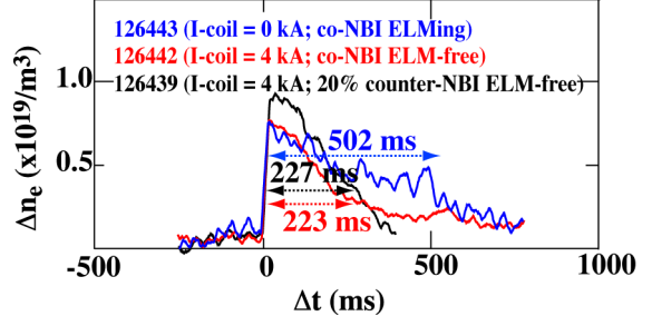
FIG. 6. Decay of pellet-induced density rises \Delta n_e in: (blue) ELMing H-mode with I-coil = 0 kA, (red) RMP-assisted ELM-free H-mode with 100% co-NBI, and (black) RMP-assisted ELM-free H-mode with 20% counter-NBI. The discharges have similar divertor recycling behavior.
