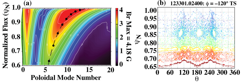
FIG. 2. (a) Color contour plot of the magnetic perturbation spectrum, showing the Fourier amplitude of the n = 3 vacuum field from a 2 kA I-coil current in discharge 122344 as a function of poloidal mode number m and normalized poloidal flux \psi_n . Contributions from measured field errors are included. White contour lines are drawn at each 10% in amplitude. Mode resonances m = nq(\psi_n) ( \bullet ) lie along a ridge in the contours of the perturbing field. The color bar shows the amplitude scale in Gauss. (b) Poincaré plot of the vacuum perturbed magnetic field in the (\theta, \psi_n) plane for \phi = -120^\circ in discharge 123301 at 2400 ms.
