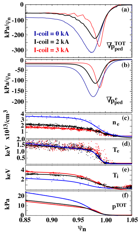
FIG. 4. (a) Pedestal total pressure gradient and (b) electron pressure gradient versus I-coil current in \delta \sim 0.37 discharges. (c) Pedestal profiles of (top to bottom) n_e , T_e , T_i , and p^{TOT} vs I-coil current. Dots are data points; lines are hyperbolic tangent fits to the data. The profile for 0 kA (blue) is obtained by fitting Thomson and CER data in the last 20% of the ELM cycle. The 2 kA (yellow) and 3 kA (red) profiles are fits to all Thomson and CER data in 500 ms windows during ELM suppression.
