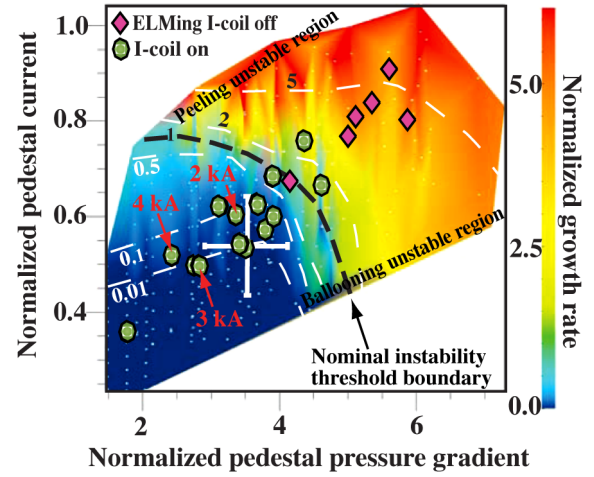
FIG. 5. Normalized P-B mode growth rates \gamma_N = \gamma/(0.5\omega_{*e}) (where \gamma is the P-B growth rate and \omega_{*e} is the electron diamagnetic drift frequency) for 6 ELMing cases (diamonds) just before an ELM and 14 RMP-induced ELM-free (ellipses) cases. \gamma_N is plotted as a function of the maximum value of the normalized pedestal pressure gradient \alpha = -[\mu_o/(2\pi)^2]\partial V/\partial\psi(V/2\pi^2R_o)(\partial p/\partial\psi) (where V is the plasma volume, p is the pressure, \psi is the poloidal magnetic flux and R_o is the major radius of the plasma) and a characteristic pedestal current density j_N^{ped} , which is taken to be the peak value of the parallel current in the pedestal normalized by the average parallel current in the pedestal. The stability boundary (black dashed line). Representative error bars, denoting one standard deviation, are shown on the data point at \alpha = 3.4 and j_N^{ped} = 0.53 . The color bar shows the value of \gamma_N for the color contours in the plot.
