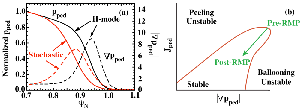
FIG. 1. (a) Schematic of ELMing H-mode (black) and RMP-assisted ELM-free H-mode (red) profiles of pedestal pressure p_{ped} (solid) and pressure gradient \nabla p_{ped} (dashed). (b) Schematic of the P-B stability diagram ( J_{ped} , |\nabla p_{ped}| ) showing how the \nabla p_{ped} drop moves the pedestal diagonally (green arrow) from the unstable to the stable region due to dependence of the bootstrap current on \nabla p_{ped} .
