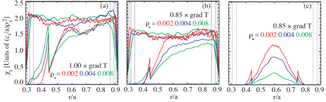
Fig. 3. Ion diffusivity normalized to gyroBohm versus radius for ITG adiabatic electron piecewise flat profiles with DIII-D r/a=0.6 parameters from Figs. 1 and 2 in (a); ion temperature lowered by 0.85 in (b) and (c). Both left and right regions are stable in (c).
