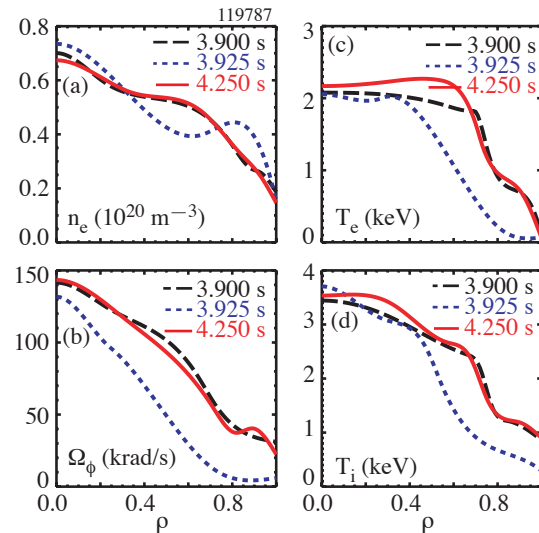
Fig. 9. Profiles of (a) electron density, (b) toroidal rotation, (c) electron temperature, and (d) ion temperature just before an ITB collapse (3.9 s, black dashed), just after the collapse (3.925 s, blue dotted), and just before the next ITB collapse (4.25 s, red solid).
