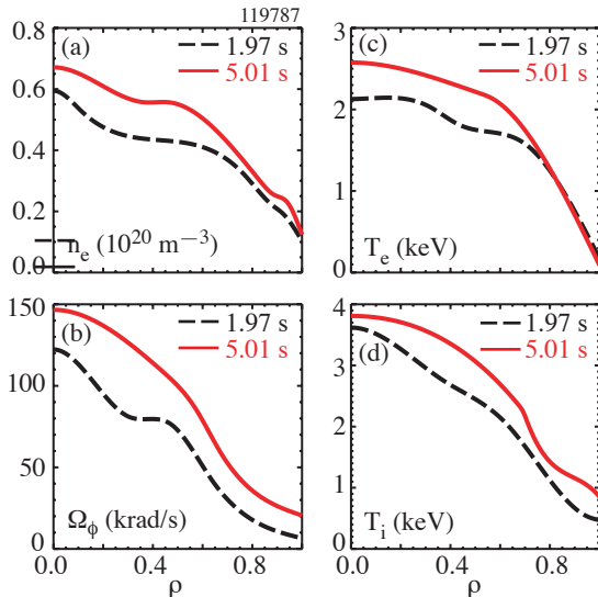
Fig. 3. Profiles of (a) electron density, (b) toroidal rotation, (c) electron temperature, and (d) ion temperature at 1.97 s (early in the discharge evolution; black dashed) and 5.01 s (near the end of the discharge; red solid).
