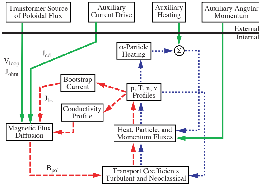
Fig.1. Nonlinear couplings in advanced tokamak transport. The blue (dotted) lines indicate the fast heat and momentum transport loops, the red (dashed) lines show the slow magnetic flux transport loop, and the green (solid) lines represent external inputs and controls. In small devices the external inputs are dominant, but in a burning plasma the external inputs will be very weak.
