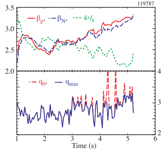
Fig. 4. Evolution of (a) \beta_p (solid), \beta_N (dashed) and the internal inductance (dotted), and (b) q(0) (dashed) and q_{min} (solid).
