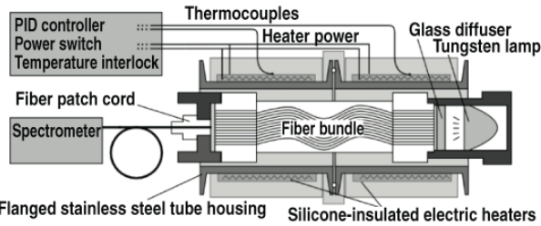
FIG. 1. Schematic representation of a fiber bundle in the baking oven with transmission instrumentation connected.
