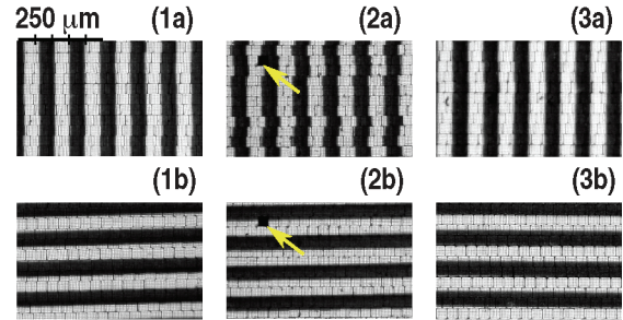
Fig. 4. Images of the same vertical and horizontal line patterns viewed through three different fiber bundles. (1a,b) are through a new, unbaked fiber bundle. (2a,b) are through a fiber bundle that was cycled twice to 200°C (once at 12 deg/h and once at 50 deg/h with 100 deg/h cooling), held for a total of 218 h, with forced air cooling of the fiber ends. (3a,b) are taken through a fiber bundle that was cycled four times to 200°C (twice at 8.3 deg/h and twice at 50 deg/h) and held for a total of 421 h, with uniform heating through the fiber ends. The yellow arrows in images 2a and 2b points to a broken multi-fiber.
