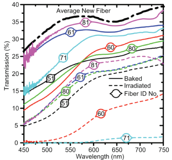
FIG. 2. Transmission spectra of a typical fiber bundle before irradiation (dash-dot), and several fiber bundles after a period of irradiation (dash), and subsequent baking (solid).
