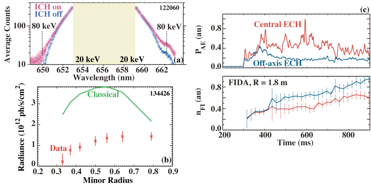
FIG. 10. Three types of physics studies. (a) Change in FIDA spectra as a parameter is changed. In this example, fast ions are accelerated when ion cyclotron heating (ICH) is applied. [Adapted and reprinted with permission from W.W. Heidbrink, et al. , Plasma Phys. Control. Fusion 49 , 1457 (2007). Copyright 2007 IOP Publishing Ltd.] (b) Comparison of the spatial FIDA profile with the profile predicted by theory. In this example, the measured profile differs dramatically from classical expectations due to fast-ion transport by drift waves. [Adapted and reprinted with permission from W.W. Heidbrink et al. , Plasma Phys. Control. Fusion 51 , 125001 (2009). Copyright 2009 IOP Publishing Ltd.] (c) Change in the time evolution of the FIDA signal as plasma parameters change. In this example, application of ECH at different locations modifies the amplitude of Alfvén eigenmode activity, which alters the fast-ion transport. [Adapted and reprinted with permission from M.A. Van Zeeland et al. , Plasma Phys. Control. Fusion 50 , 035009 (2008). Copyright 2008 IOP Publishing Ltd.]
