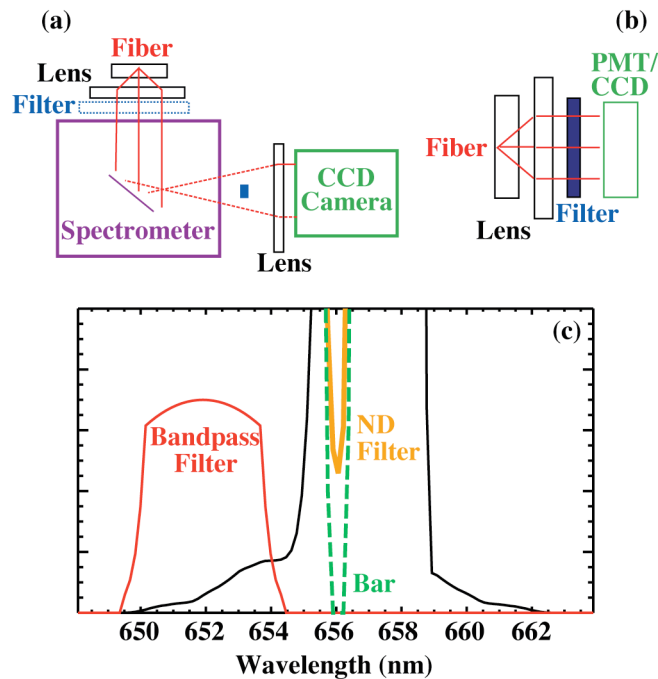
FIG. 5. Schematic illustrations of (a) the spectroscopic approach to a FIDA measurement, (b) the bandpass-filtered approach, and (c) the resulting effect on the spectrum. In a spectroscopic measurement, light that is dispersed by a spectrometer is measured with a CCD camera. If the full spectrum is measured, a neutral density filter [orange line in (c)] or blocking bar [dashed line in (c)] placed in the focal plane between the spectrometer and camera attenuates the intensity of the cold D_\alpha line. If only one side of the spectrum is measured, a filter at the entrance to the spectrometer attenuates the cold D_\alpha line. In a f-FIDA or two-dimensional imaging application, a bandpass filter selects the desired spectral band [red curve in (c)] before detection by a photomultiplier or CCD camera.
