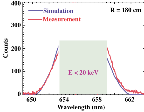
FIG. 8. Comparison of the measured FIDA spectrum with the predicted spectrum in an MHD-quiescent DIII-D plasma. For small Doppler shifts ( E_{\lambda} < 20 keV), uncertainties in the background subtraction are large. [Reprinted with permission from Y. Luo et al. , Phys. Plasmas 14 , 112503 (2007). Copyright 2007, American Institute of Physics.]
