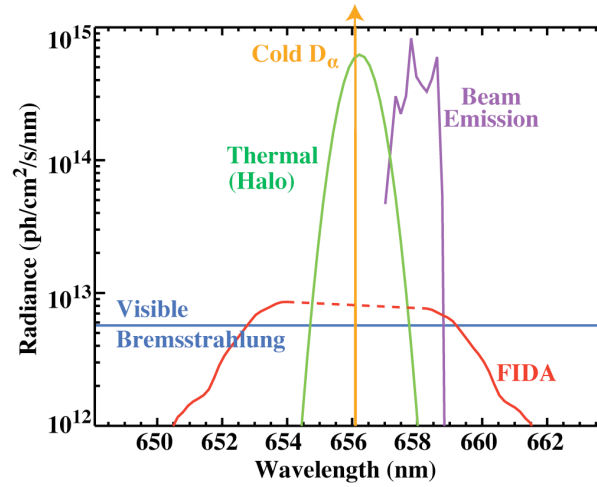
FIG. 3. Various sources of light in the D_\alpha spectral band for a typical case. The spectral intensity of D_\alpha light from edge neutrals is largest. Radiation from injected neutrals and from halo neutrals are an order of magnitude larger than the FIDA and visible bremsstrahlung spectral features.
