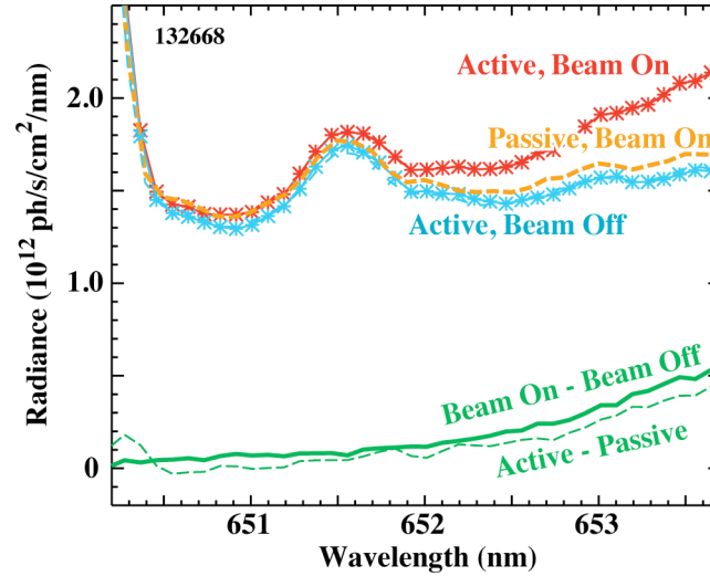
FIG. 4. Comparison of different methods of background subtraction for an NSTX discharge with average beam power of only 0.5 MW. The blue-shifted side of the spectrum is shown. The two spectra labeled “Active, Beam On” and “Active, Beam Off” are from a fiber that views the injected neutral beam; the difference of these signals is the FIDA spectrum obtained from beam modulation and is labeled “Beam On - Beam Off”. The dashed line labeled “Passive, Beam On” is from a toroidally separated view acquired when the injected beam is on. (A slight difference in passive signal is observed during beam modulation.) The dashed FIDA spectrum labeled “Active-Passive” is obtained using this signal to subtract the background. Passive impurity lines at 650.0 and 651.5 nm are evident in the raw spectra but disappear upon background subtraction.
