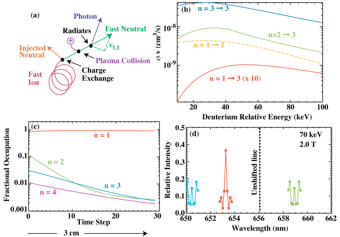
FIG. 1. (a) The FIDA process. A fast ion traverses a neutral beam and is neutralized in a charge exchange reaction. The atomic energy levels change while the neutral propagates. Some neutrals radiate a D_\alpha photon that is Doppler shifted by the velocity component in the direction of emission. (b) Charge exchange reactivities for transitions from various energy levels to the n=3 level. The abscissa is the relative energy between the ion and neutral computed from the relative velocity. Note that transitions from the ground state are ten times less probable than shown. (c) Time evolution of level occupations obtained from solution of the collisional-radiative transition equations for 80-keV neutrals in a DIII-D discharge. The neutral only travels a few centimeters before the n=3 occupation level decays to a negligible level. (d) Sample of spectra from 70-keV neutrals for various velocity vectors relative to the photon and magnetic-field directions. The shift from 656.1 nm (dashed line) is due to the Doppler shift; the line splitting is caused by the motional Stark effect.
