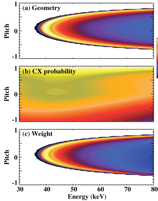
FIG. 6. FIDA weight function W vs. energy and pitch for a nearly vertical view in DIII-D. The contours are on a linear scale for a blue-shifted wavelength corresponding to E_\lambda = 40 keV (a) Contribution to the weight function associated with measuring a single component of the velocity. (b) Contribution to the weight function associated with variations in neutralization probability. (c) Total weight function W .
