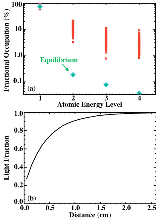
FIG. 2. (a) Distribution of initial energy levels ( x ) for an ensemble of reactions in DIII-D discharge #132607. 8 The diamond symbols represent the equilibrium distribution of states at the same location in the plasma. (b) Distance traveled by the atom before radiating a D_\alpha photon for the distribution shown in (a). (The calculation includes the charge-exchange reaction probabilities for the various initial conditions.) Nearly all of the light is emitted within a distance of 2 cm.
