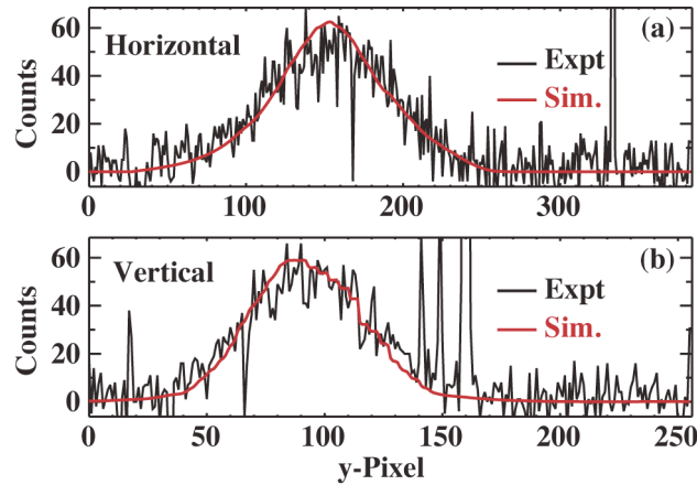
FIG. 9. Comparison of DIII-D FIDA imaging data with the predicted profile for (a) horizontal and (b) vertical lines through the maximum of the measured image. [Adapted and reprinted with permission from M.A. Van Zeeland et al. , Plasma Phys. Control. Fusion 51 , 055001 (2009). Copyright 2009 IOP Publishing Ltd.]
