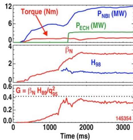
Fig. 2-4. High fusion performance at low torque.
