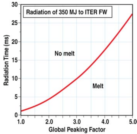
Fig. 2-31. Requirements for thermal energy deposit on the ITER first wall.
