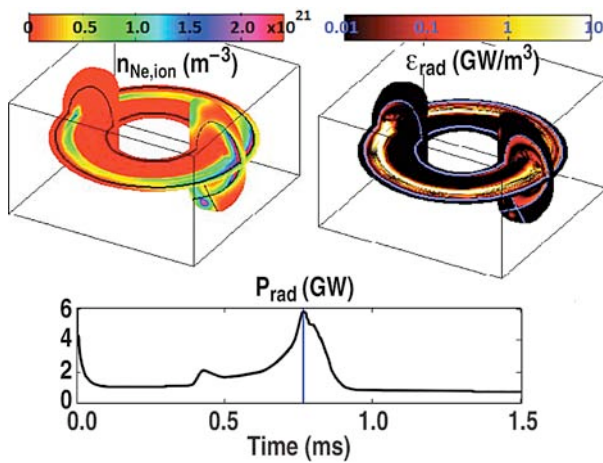
Fig. 2-33. NIMROD 3D MHD modeling of DIII-D thermal energy radiation from MGI. Note the precursor reconnection event at \sim 0.4 ms.
