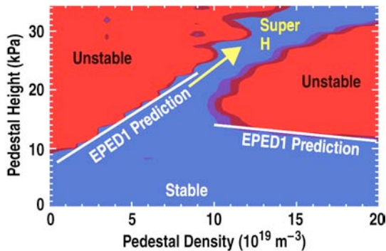
Fig. 4-10. Studies with the EPED model predict that there is stable access to very high pedestal pressures in some pedestals. Achieving these pressures imposes strong requirements on how pedestal pressure and density must simultaneously evolve [Snyder 2012a].
