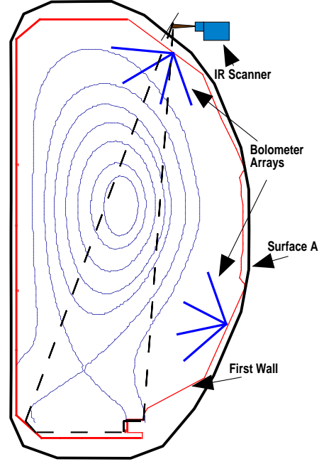
Fig. 1 A cross sectional view of DIII-D showing the poloidal locations and tokamak views of the IR scanners and bolometer arrays. The outermost line denotes Surface A. The line labeled First Wall denotes the plasma facing carbon armor surface. Not shown is the vacuum vessel inner wall which lies just outside Surface A.
