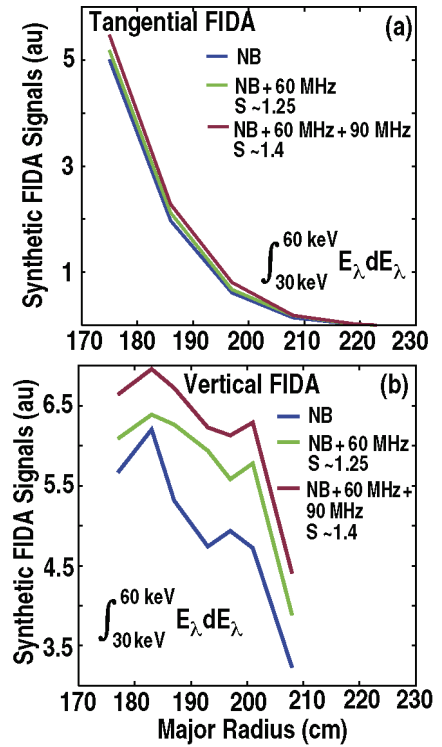
Fig. 3. Computed FIDA signals for (a) tangential FIDA and (b) vertical FIDA for NB only (blue), NB + 60 MHz (green) and NB + 60 MHz + 90 MHz (red).
