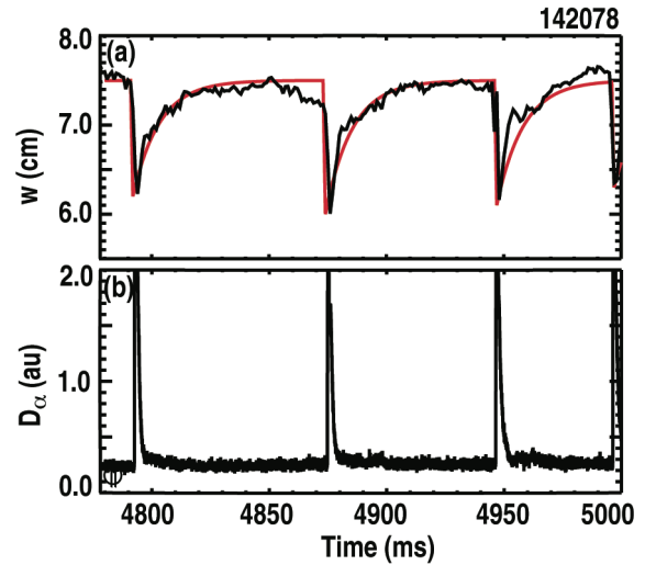
Fig. 3. For ELM-TM coupling events, (a) (black) measured island width (red) analytical expression for the recovery given by Eq. (2). (b) Filterscope measurement of ELM induced D_\alpha emissions.
