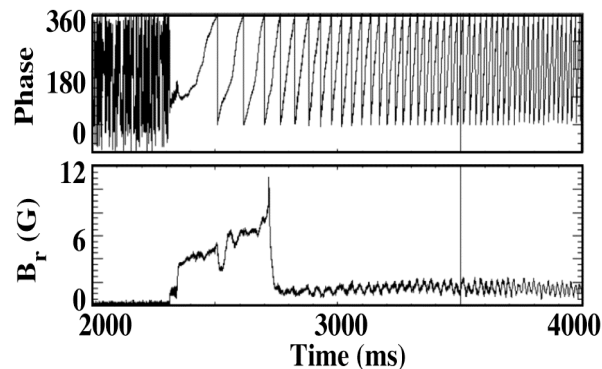
Fig. 2. Phase and amplitude of an NTM initially locked to the wall which is then locked to the I-coil at t = 2400 ms and forced to rotate by the I-coil traveling wave accelerating from 1 to 60 Hz. DIII-D #126685.
