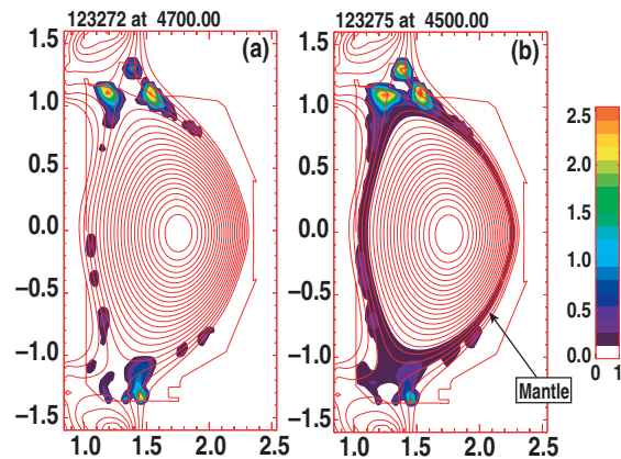
Fig. 3. Tomographic inversions of bolometer data show the poloidal distribution of the radiated power density for (a) Case 1 and (b) Case 3.
