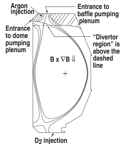
Fig. 1. Particle pumping- and gas injection locations are superimposed on the plasma cross-section. The “divertor region” lies above the dashed line.
