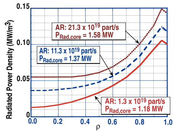
Fig. 2. The radiated power densities for the three D_2 + argon injection cases are plotted as a function of normalized radial coordinate \rho .
