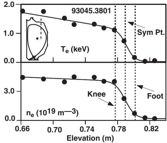
Fig. 1. Typical profiles of T_e and n_e in the H-mode pedestal. Data shown as function of vertical position along Thomson chord, measured relative to midplane of machine. Solid lines are fits from tanhfit function. Positions of density foot, symmetry point and knee are shown as vertical lines. Inset shows Thomson laser chord.
