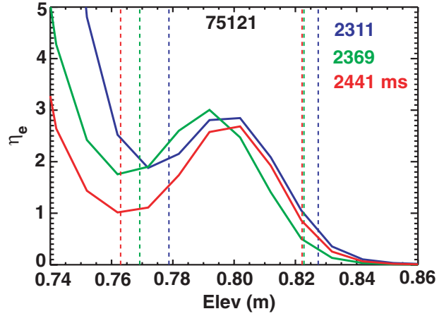
Fig. 4. Profiles of \eta_e along Thomson laser at three different times in the ELM-free phase of a VH-mode discharge. Vertical lines show locations of knee and foot of density profile (lower and higher elevation, respectively).
