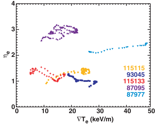
Fig. 3. Plot of \eta_e and \nabla T_e , measured at point of steepest density gradient during ELM-free phases of discharges. Various discharges are differentiated by color and symbol. Gradient is along Thomson laser path.
