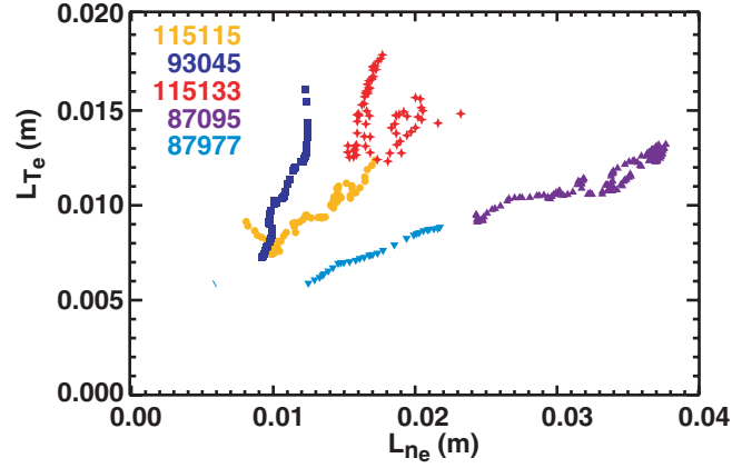
Fig. 2. Plot of L_{T_e} and L_{n_e} data, measured at point of steepest density gradient during ELM-free phases of discharges. Various discharges are differentiated by color and symbol. Scale lengths are along Thomson laser path.
