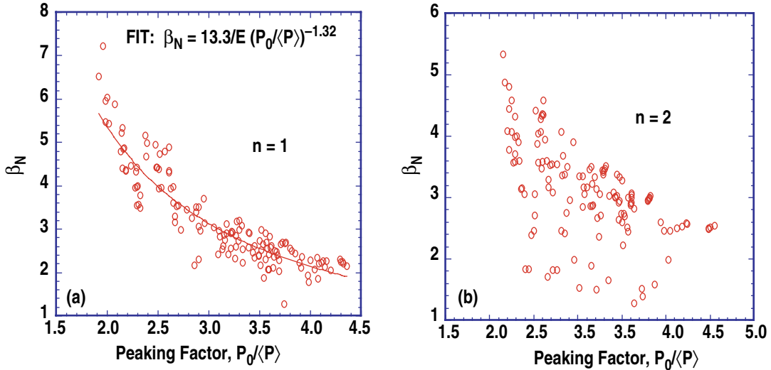
Fig. 1. Limiting \beta_N values for the n = 1 (a) and n = 2 (b) ideal modes as a function of P_0/\langle P \rangle for all combinations of \kappa , \delta , \zeta_0 , and peaking factor.
