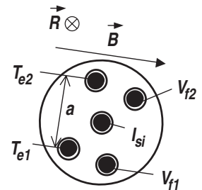
Fig. 1. Probe head layout.
