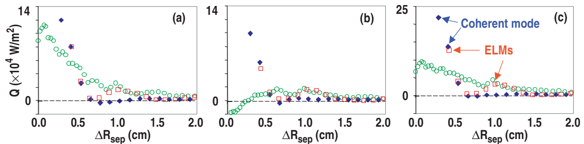
Fig. 4. Radial profiles of convective (a), conductive (b), and total (c) heat fluxes in L-mode (open circles), ELM-free H-mode (solid diamonds), and ELMy H-mode (open squares).
