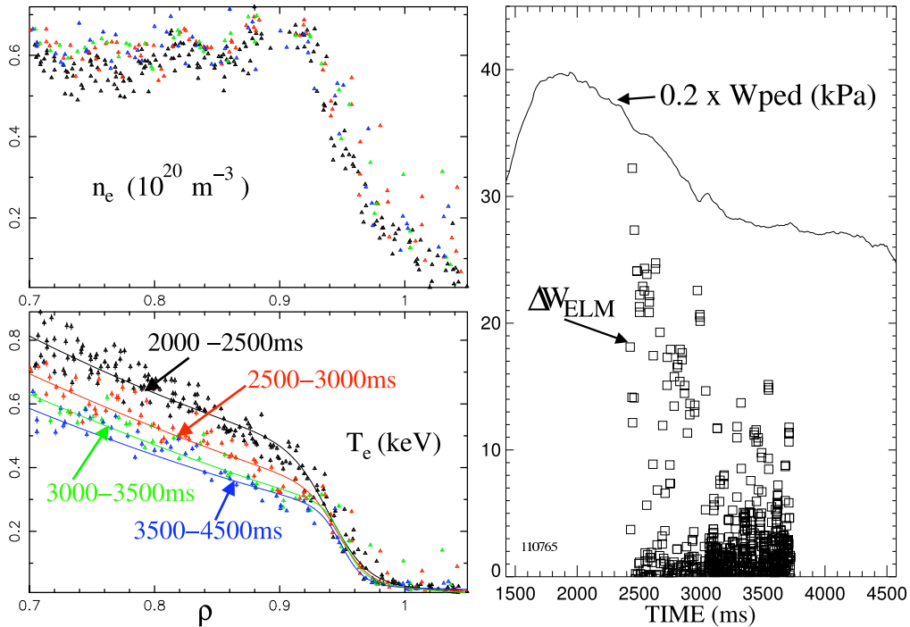
Fig. 2: Width of the steep gradient region in the temperature profile narrows as the H-mode pedestal energy and ELM energy loss are reduced in a discharge with continuous D2 puffing and n_e^{PED} / n_{GW} = 0.75 .
