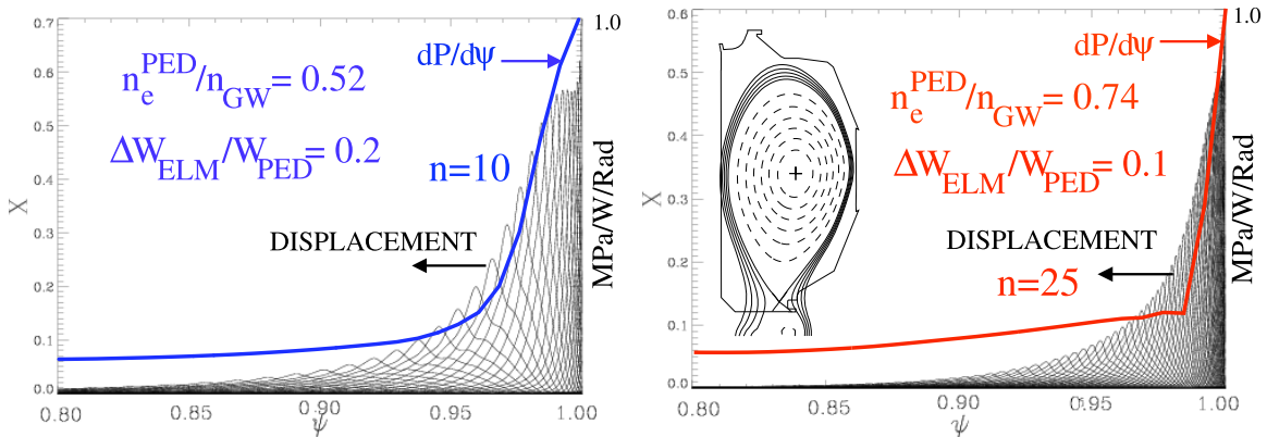
Figure 3: Comparison of peeling-ballooning eigenmode structure for low and high-density discharge showing shrinking of mode width and increase in n for high density case with narrower high p' region.
