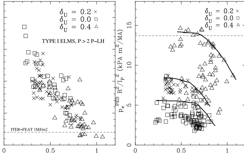
Fig. 1: a) Type I ELM energy loss normalized to H-mode pedestal pressure decreases strongly with increasing pedestal density independent of triangularity b) pedestal pressure normalized to ballooning mode decreases with increasing density and is largest at high triangularity. Approximate requirements for ITER-FEAT are given as dashed lines
