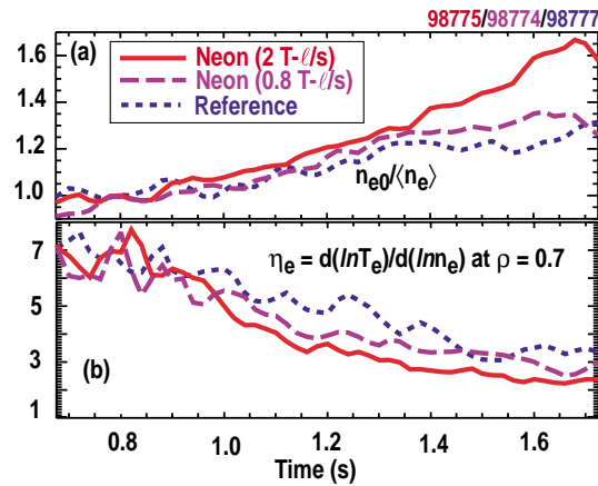
Fig. 5. Time evolution of (a) density peaking factor and (b) \eta_e (ratio of electron temperature and density gradients).
