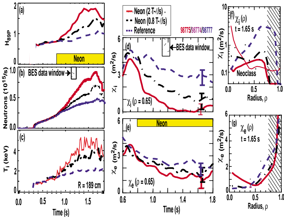
Fig. 1. Characteristics of plasma parameters for discharges with full neon (solid), half neon (chain) and a reference discharge without neon (dashed): (a) energy confinement enhancement factor, (b) neutrons, (c) central ion temperature, (d) evolution of ion and (e) electron thermal diffusivity at \rho = 0.65 , (f) ion and (g) electron thermal diffusivity profiles at t=1.65 s. The error bars in (d) and (e) represent uncertainty in assigning the convection power. The shaded area for \rho > 0.8 in (f) and (g) represents power balance uncertainties.
