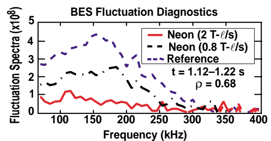
Fig. 2. Effects of varying neon quantity on BES spectra.
