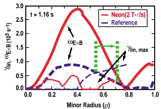
Fig. 3. Comparison of maximum linear growth rates (fine) and E \times B shearing rates (bold) in a neon-injected (solid) and reference (dashed) discharge at t = 1.16 s.
