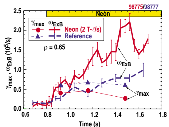
Fig. 4. Time evolution of the E \times B shearing rates (curves with error bars) and maximum linear growth rates (curves with solid circles and triangles) in a neon-injected and reference discharge.
