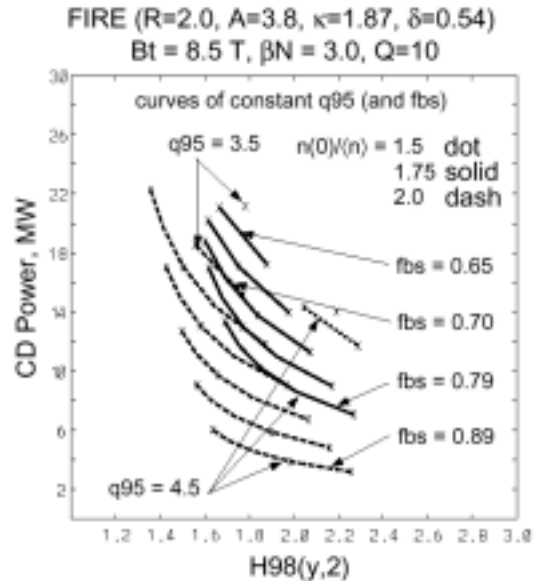
FIGURE 1. The required current drive power versus the required H98 confinement multiplier for plasmas at B_t = 8.5 T, \beta_N = 3.0 , and Q=10 . Three peak to average densities, and several q_{95} and f_{bs} values are displayed, showing accessible plasmas in the device. Similar curves would exist for other values of B_t , \beta_N , and Q .
