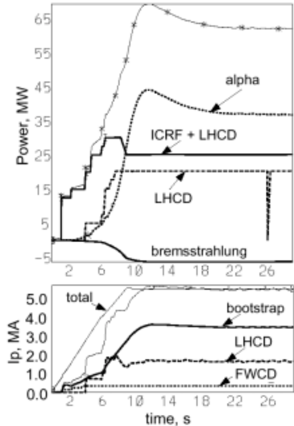
FIGURE 4. Time histories from the TSC-LSC AT simulation, of the various contributions to the plasma current and the powers injected into the plasma. The simulation is stopped after 29 s to expand the rampup phase.
