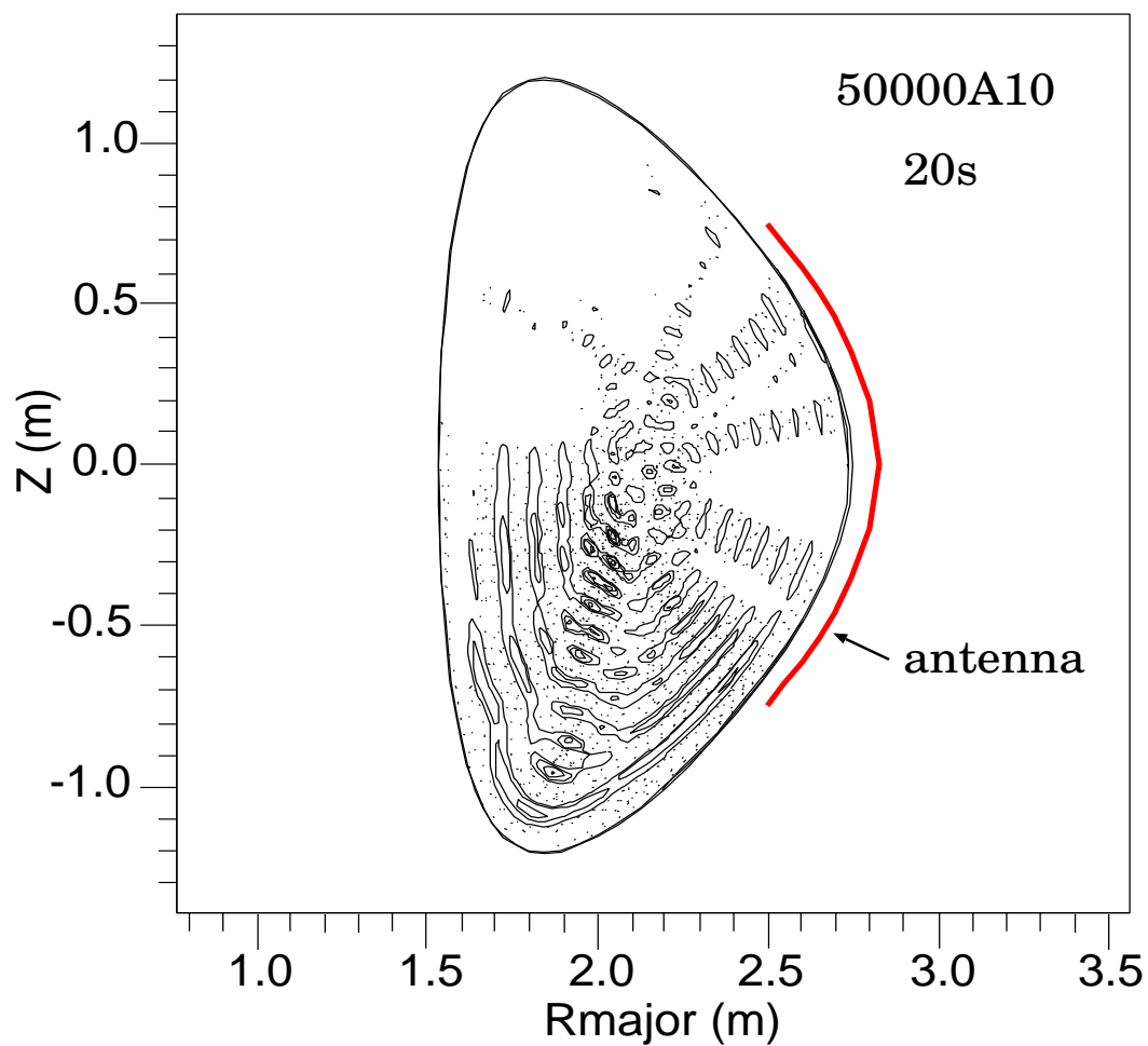
Figure 10. Contours of ICRH-induced \text{Re}\{E_r\} in the FIRE plasma.
