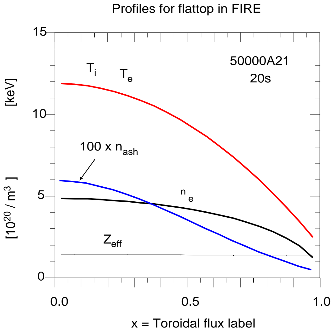
Figure 9. Profiles of the FIRE plasma in the flattop phase. The \text{He}^4 ash density times 100 is computed from the fast alpha thermalization assuming R_{ash} = 20\% and D_{ash} = 0.1 [m^2/s] , and is in steady state at the time shown.
