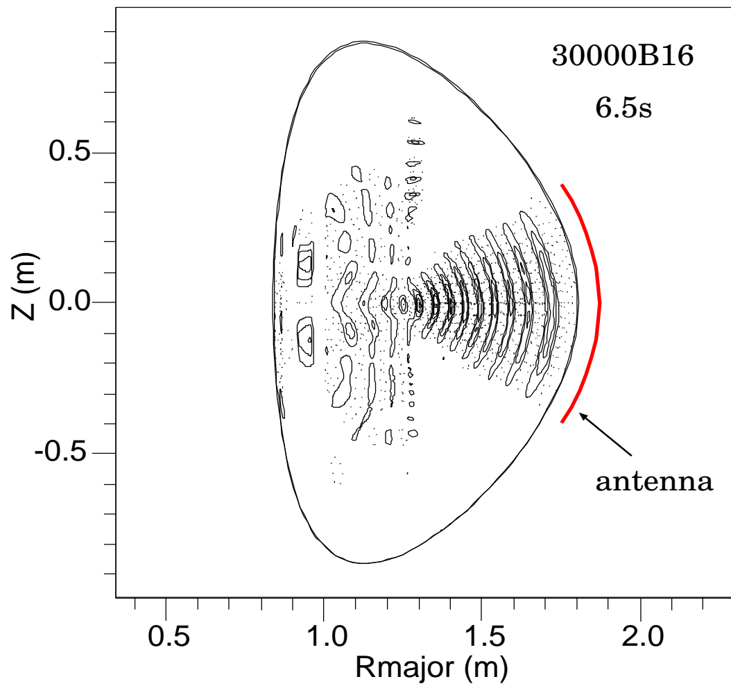
Figure 7. Contours of the ICRH-induced \text{Re}\{E_r\} in the IGNITOR plasma.
