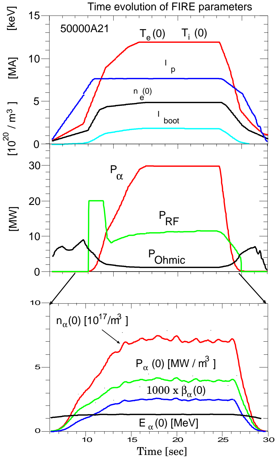
Figure 11. Time evolution of parameters in the FIRE plasma. P_{RF} is high early to obtain the L-H mode transition, then is reduced.
