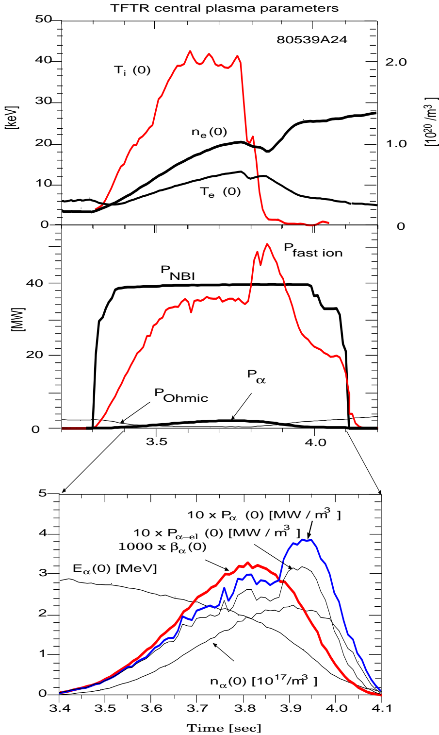
Figure 3. Time evolution of parameters in the TFTR supershot. The measured T_i profile (for carbon) became hollow with unrealistically low central values after the density became too high for good beam penetration. P_{fast\ ion} is the heating power of the thermal plasma from the NBI and alphas. E_\alpha is the average energy of the fast alphas in the core. The alpha parameters in c) are volume-averaged out to the x = 0.1 flux surface to reduce Monte Carlo fluctuations.
