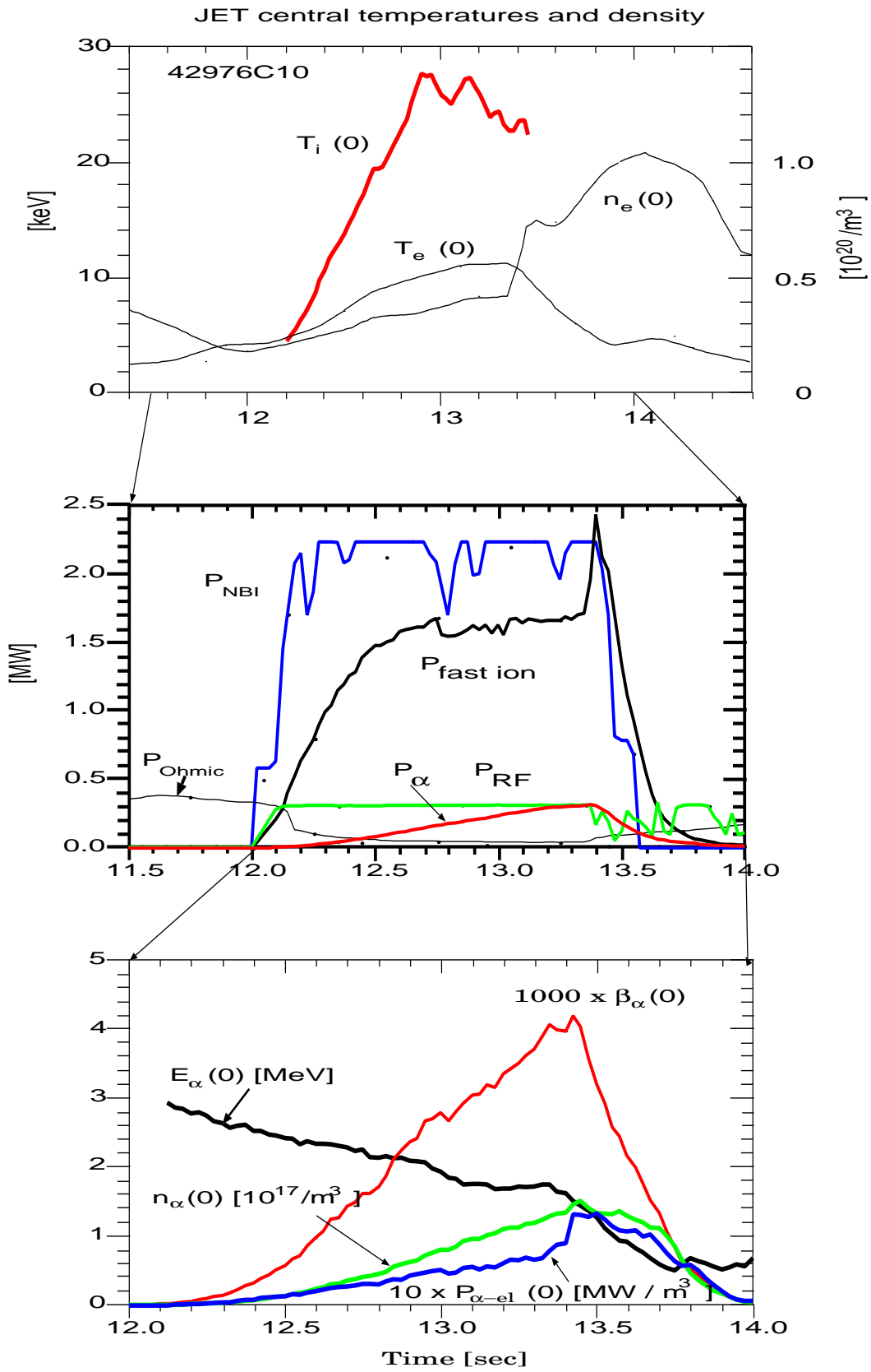
Figure 5. Time evolution of parameters in the JET plasma.
