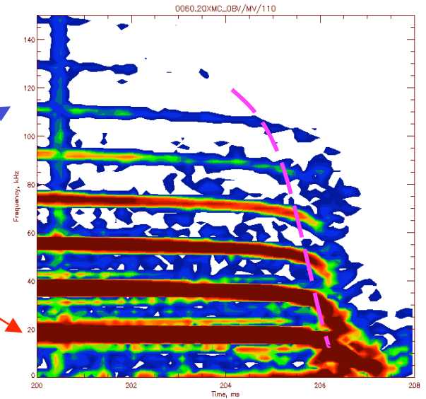
Spectrogram of outboard Mirnov
