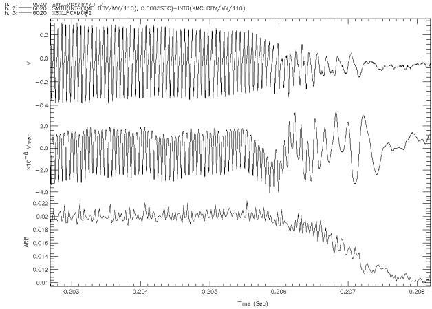
Shot # 6020. Non-integrated outboard Mirnov, integrated outboard Mirnov and SXR HCAMU2
