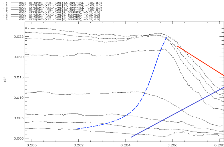
Shot # 6020. Vertical SXR signals, showing that decrease in SXR starts from periphery (higher harmonics).
